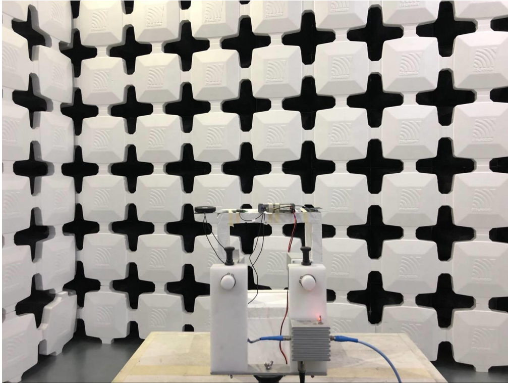
7. Radiated Emissions (Part 15C&15E) (18GHz-26.5GHz,EUT-H)
