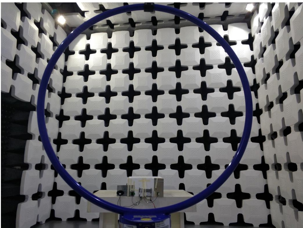
4. Radiated Emissions (Part 15C&15E 9kHz-30MHz,EUT-V)
