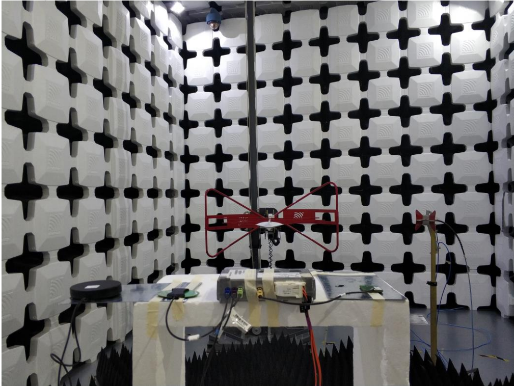
5. Radiated Emissions (Part 15C&15E 30M-18GHz,EUT-H)
