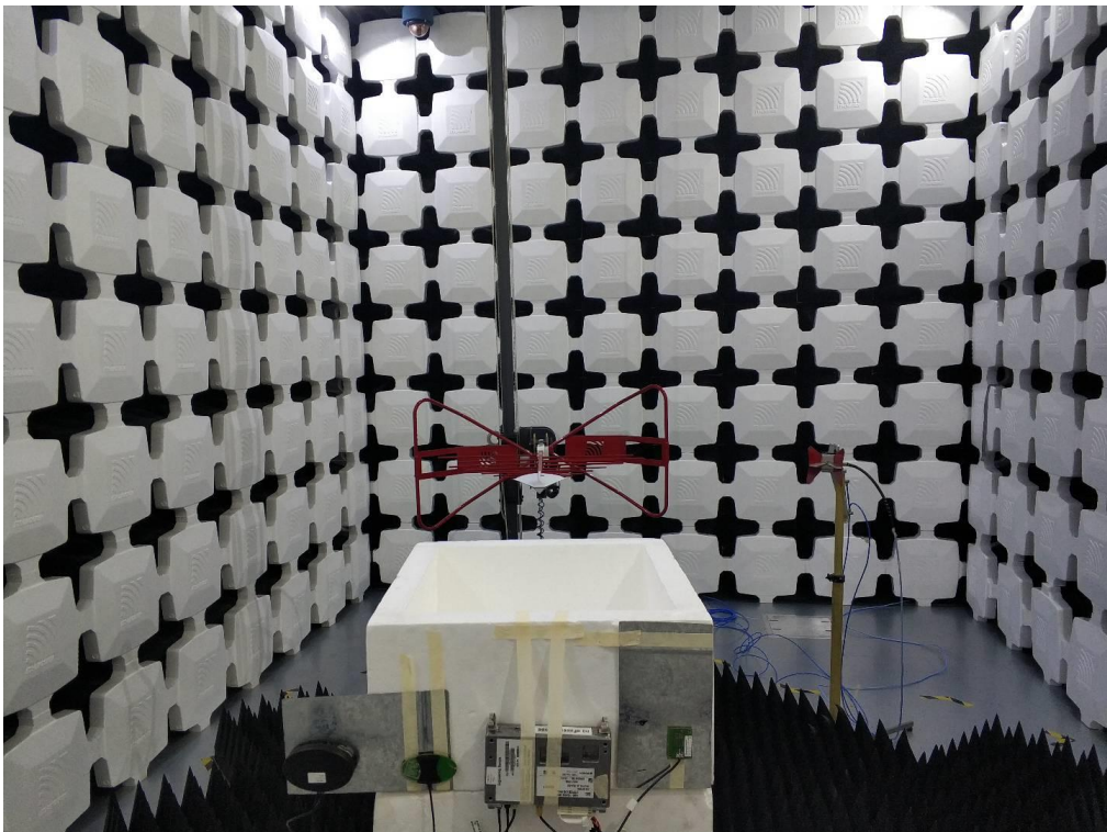
6. Radiated Emissions (Part 15C&15E 30M-18GHz,EUT-V)
