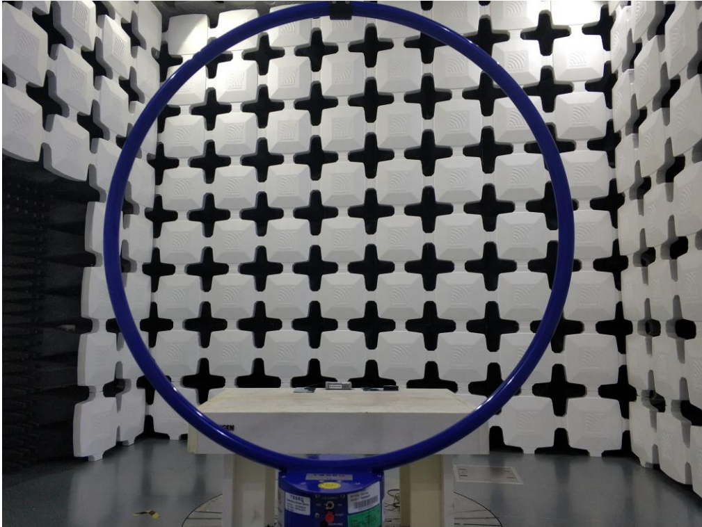
3. Radiated Emissions (Part 15C&15E 9kHz-30MHz,EUT-H)
