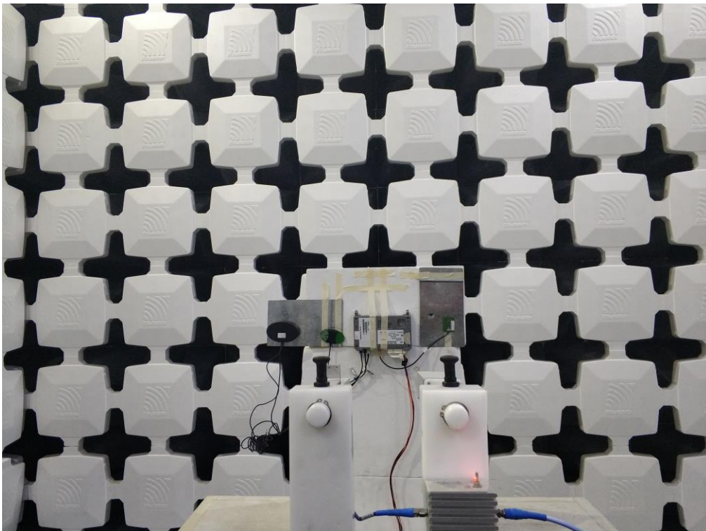
8. Radiated Emissions (Part 15C&15E) (18GHz-26.5GHz,EUT-V)
