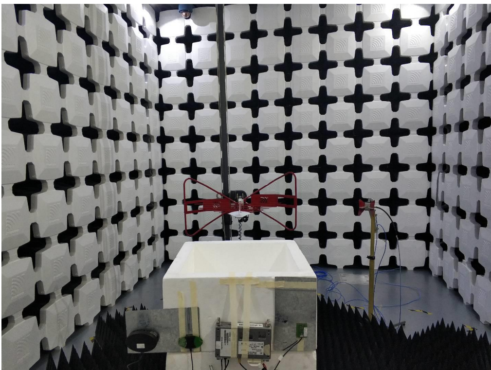
10. Radiated Spurious Emissions (30M-18GHz,EUT-V)
