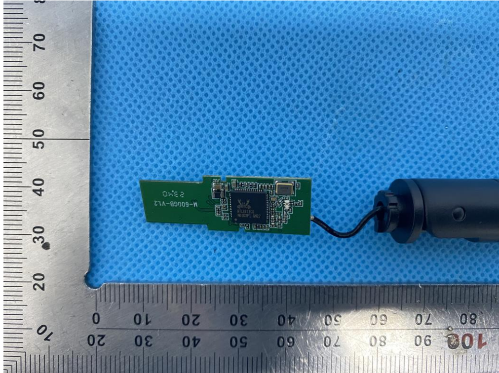
Model: XHT3510 OPEN VIEW OF EUT (FIGURE 1)
