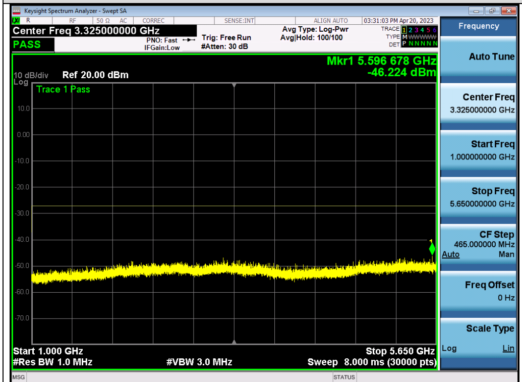
Test_Graph_802.11ax20_ANT1_5745_MCS0_Frequency Band2
