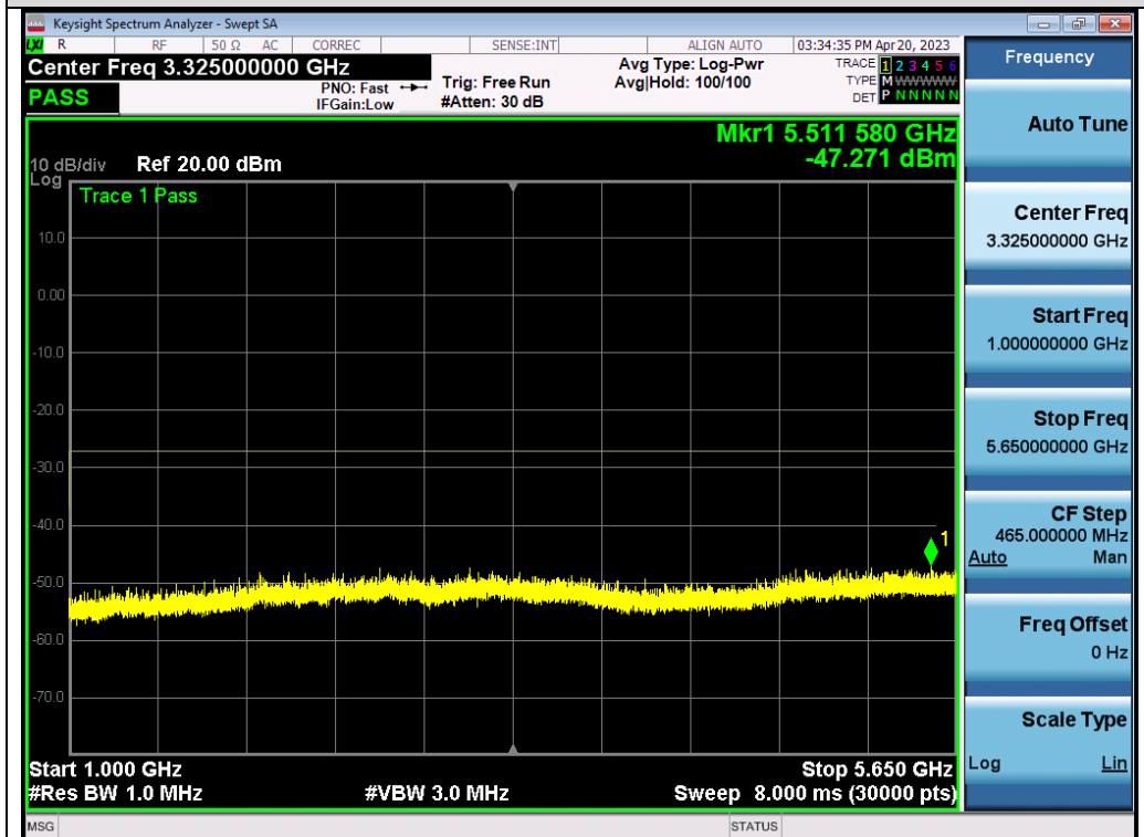
Test_Graph_802.11ax20_ANT1_5825_MCS0_Frequency Band2
