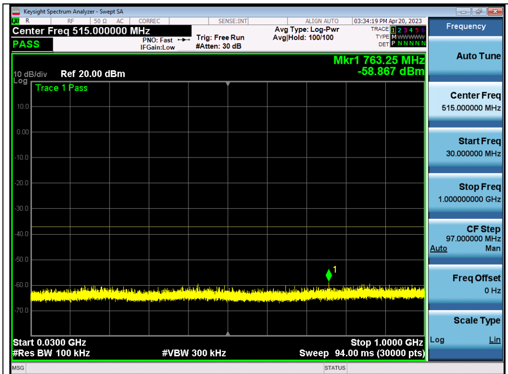
Test_Graph_802.11ax20_ANT1_5825_MCS0_Frequency Band1
