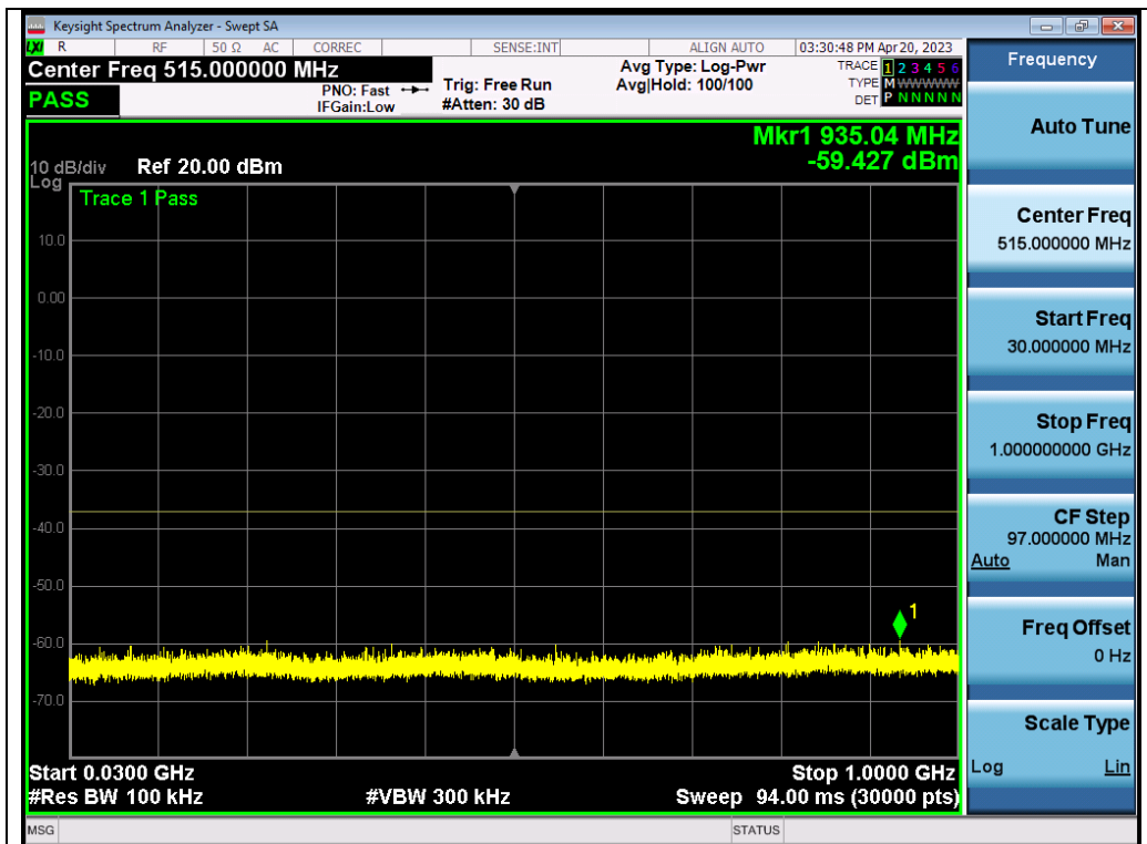
Test_Graph_802.11ax20_ANT1_5745_MCS0_Frequency Band1
