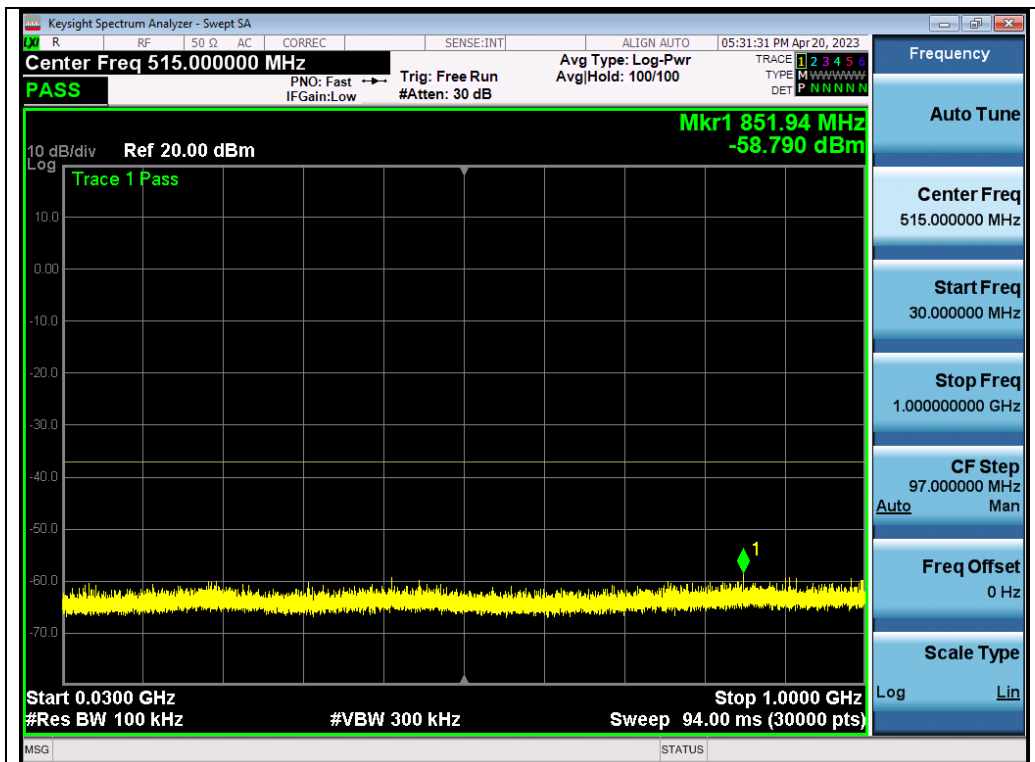
Test_Graph_802.11ax20_ANT2_5825_MCS0_Frequency Band1
