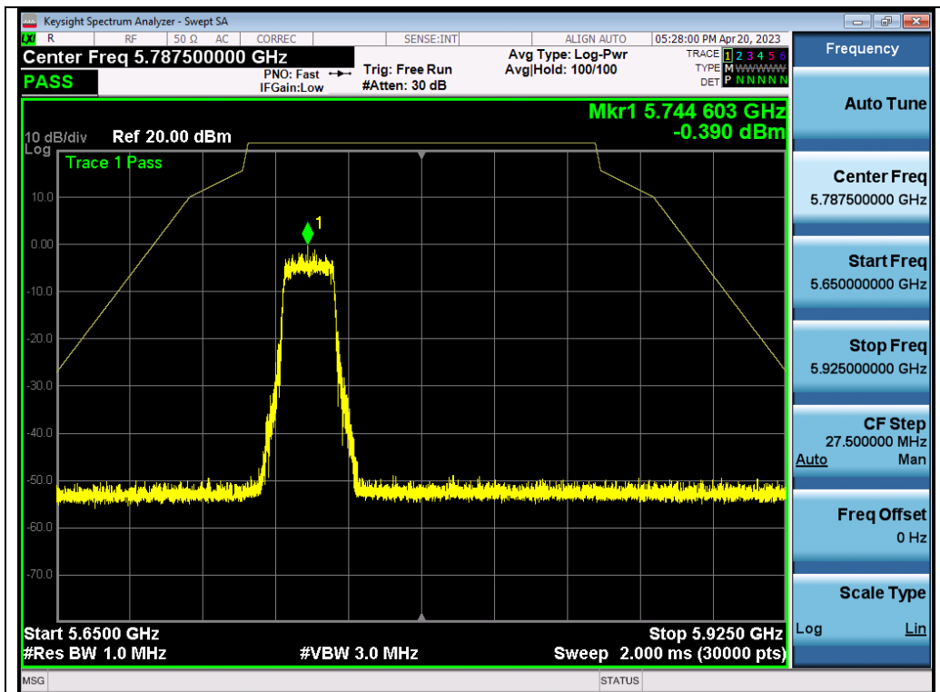
Test_Graph_802.11ax20_ANT2_5745_MCS0_Frequency Band3
