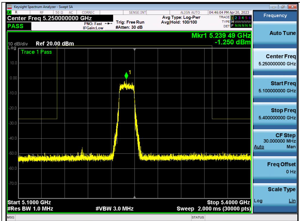
Test_Graph_802.11ax20_ANT2_5240_MCS0_Frequency Band 3
