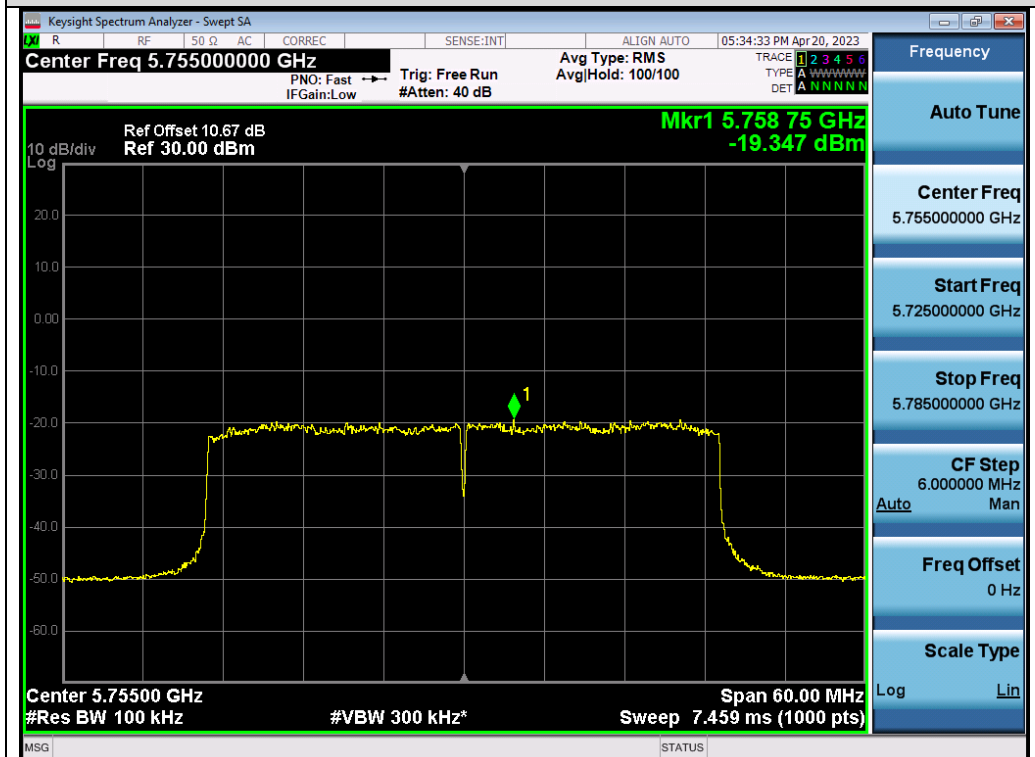
Test_Graph_802.11ax40_ANT2_5755_MCS0_PSD
