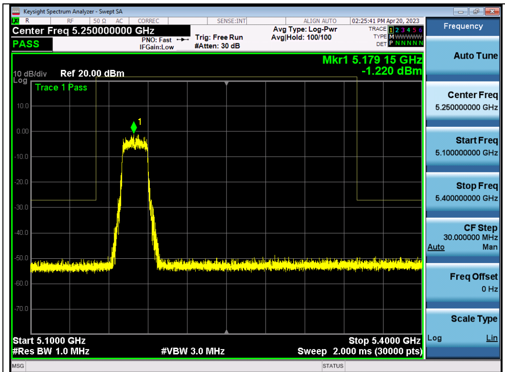
Test_Graph_802.11ax20_ANT1_5180_MCS0_Frequency Band 3
