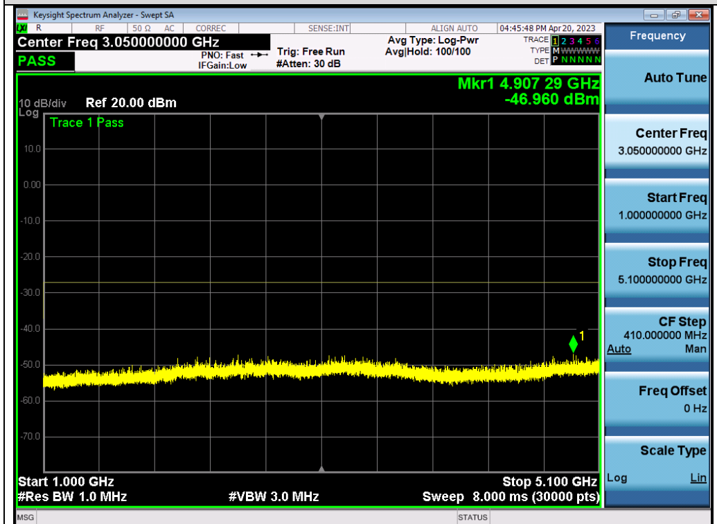
Test_Graph_802.11ax20_ANT2_5240_MCS0_Frequency Band 2
