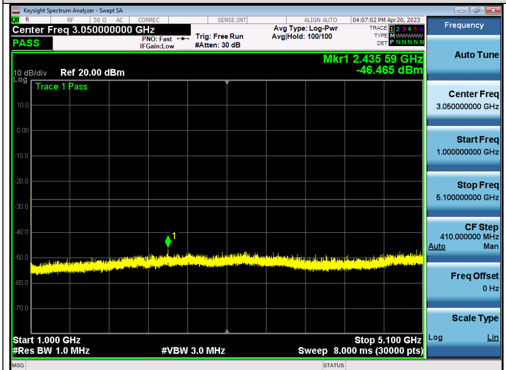
Test_Graph_802.11a_ANT2_5240_6Mbps_Frequency Band 2
