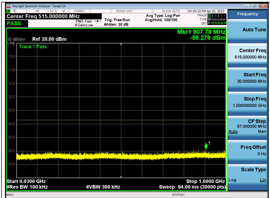
Test_Graph_802.11ax20_ANT2_5240_MCS0_Frequency Band 1
