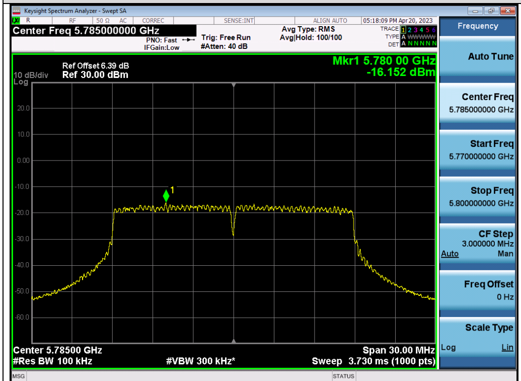
Test_Graph_802.11ac20_ANT2_5785_MCS0_PSD
