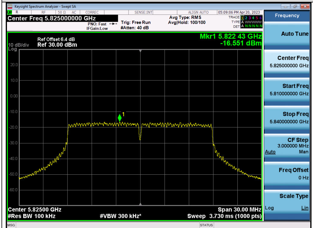
Test_Graph_802.11n20_ANT2_5825_MCS0_PSD
