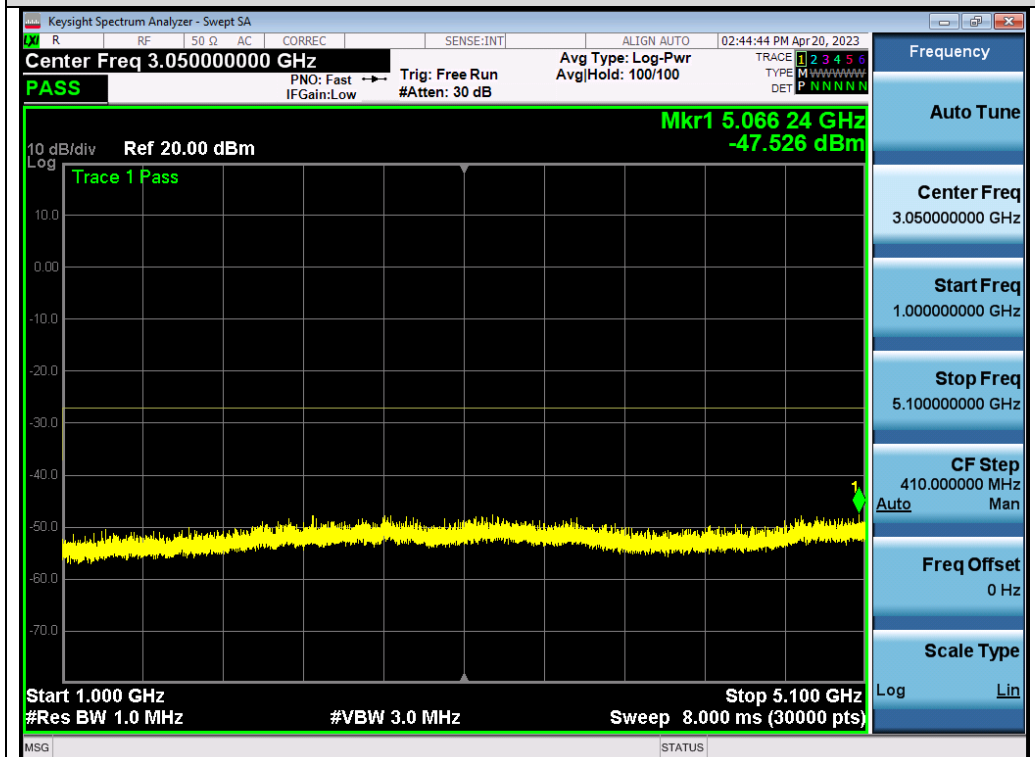
Test_Graph_802.11ax20_ANT1_5240_MCS0_Frequency Band 2
