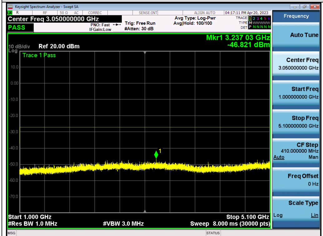
Test_Graph_802.11n40_ANT2_5230_MCS0_Frequency Band 2
