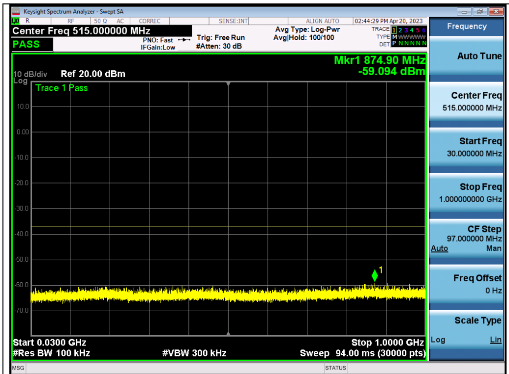
Test_Graph_802.11ax20_ANT1_5240_MCS0_Frequency Band 1
