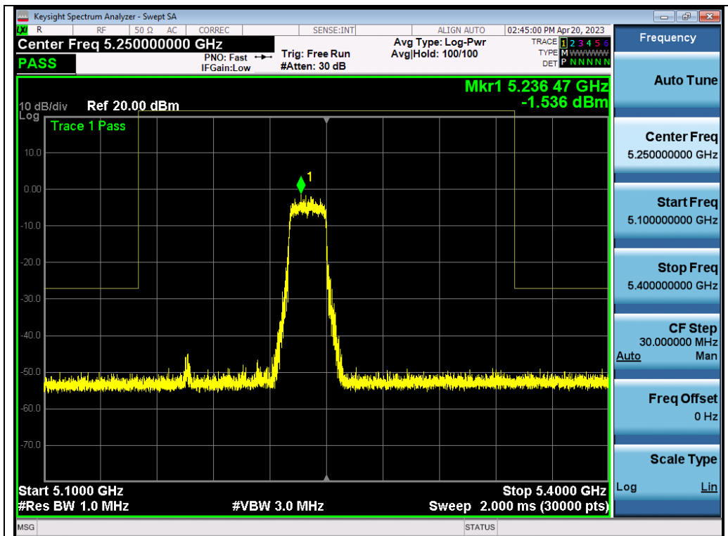
Test_Graph_802.11ax20_ANT1_5240_MCS0_Frequency Band 3
