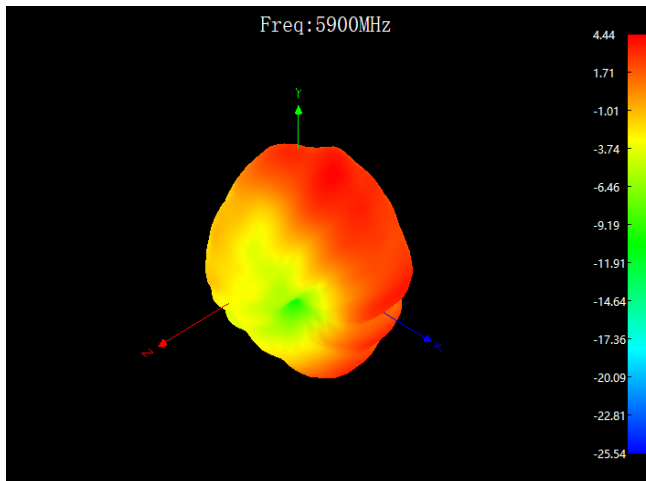
Antenna 2
