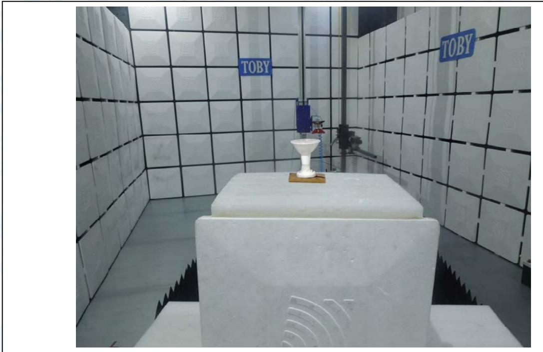
Photo of Setup for Radiated Emission (Above 1 GHz)
