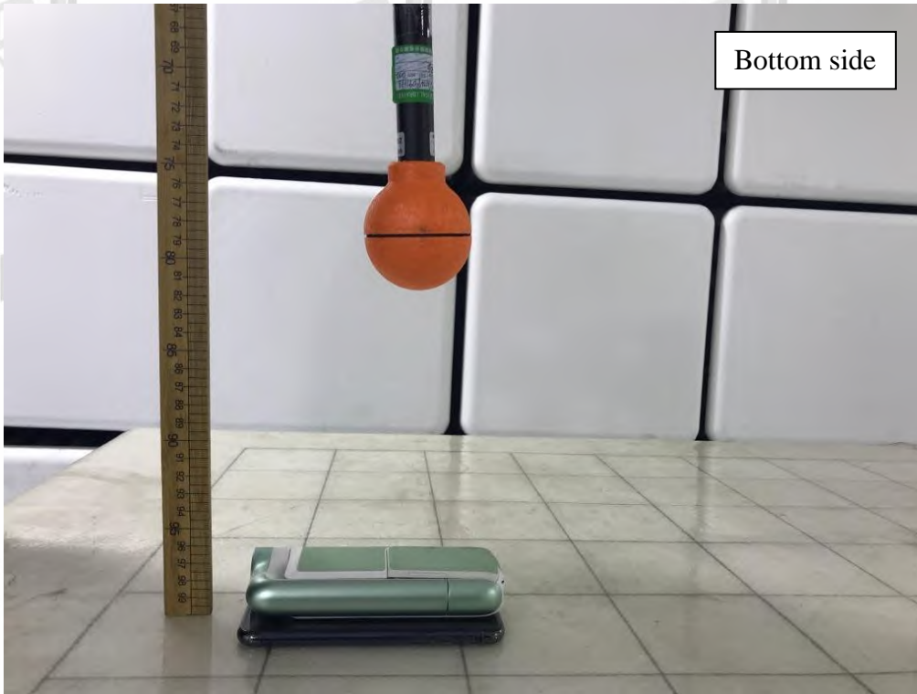
Measured distance is 20 cm for E Field
