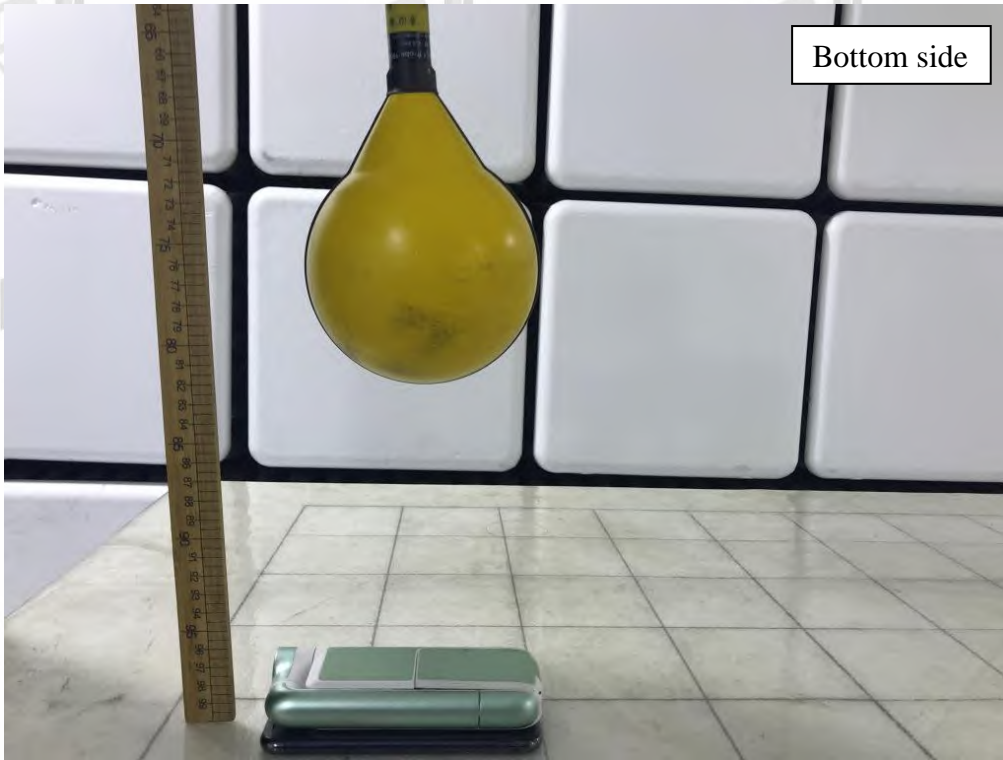
Measured distance is 20 cm for H Field
