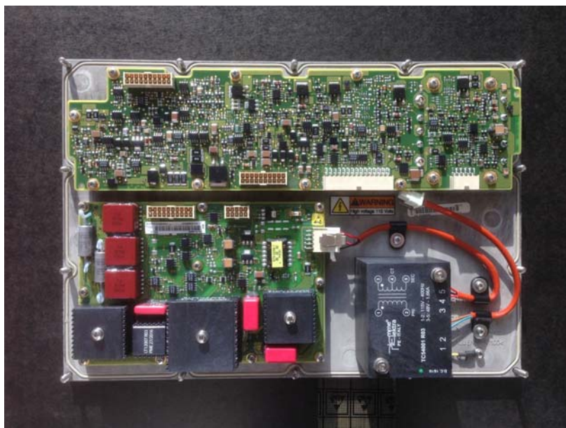
DPIO board
