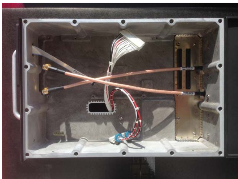
Wired Chassis RF side
