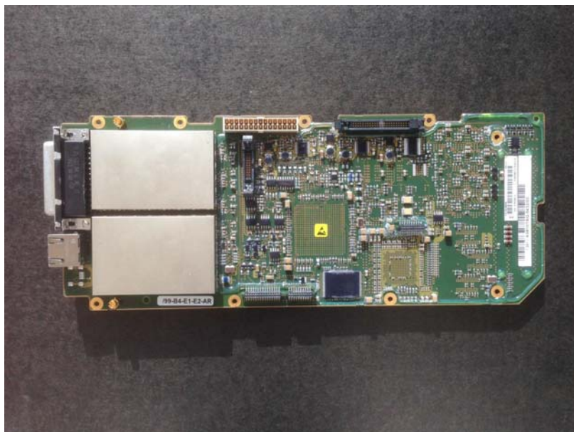
DPIO board
