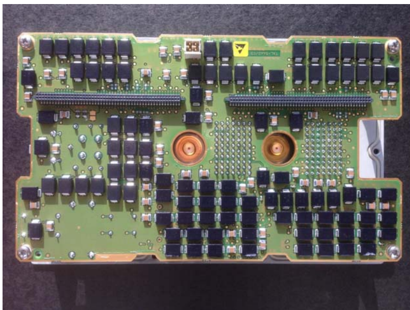
System Connector board
