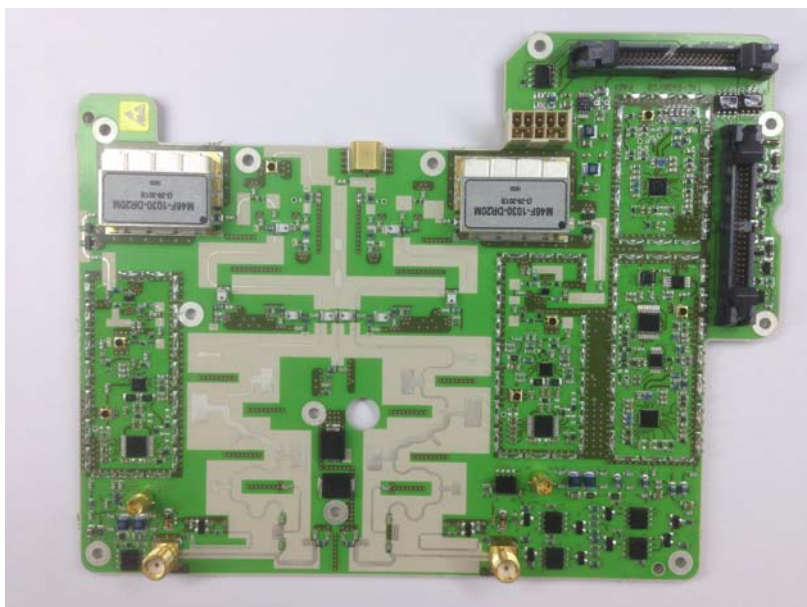
RFFE board without Shield Covers
