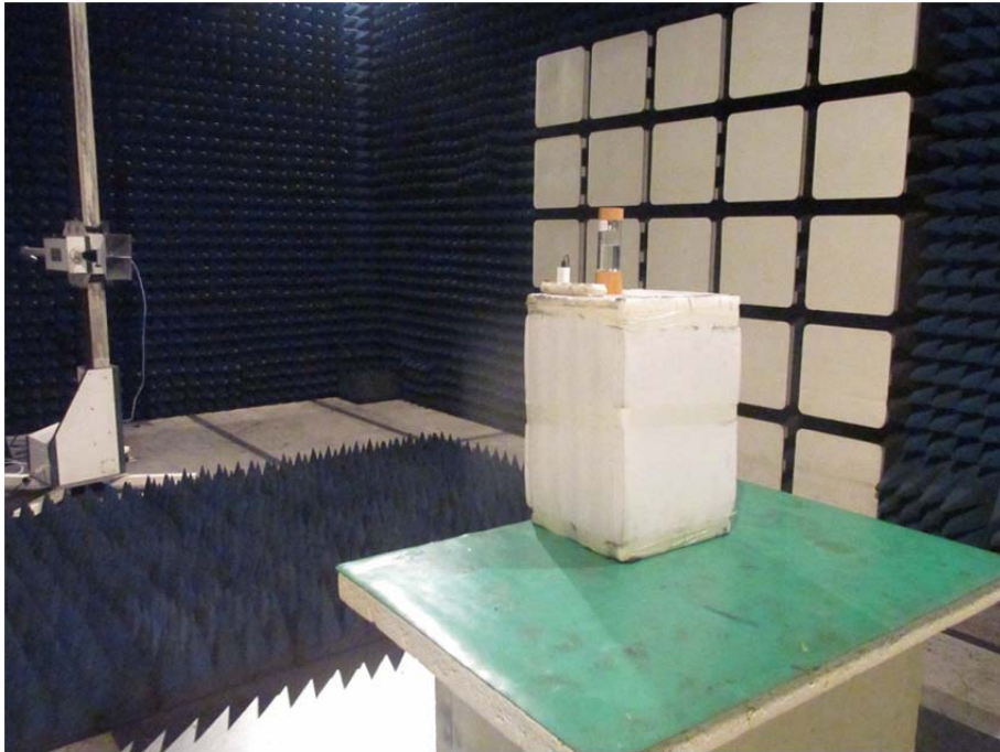
Test setup Radiation Emission
