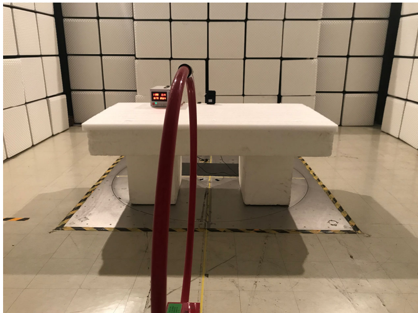
Radiated Emissions-perpendicular view (Below 30 MHz)
