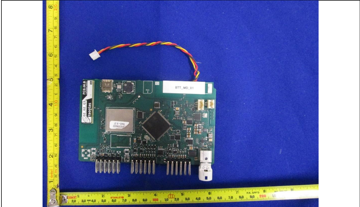
EUT Antenna Top View
