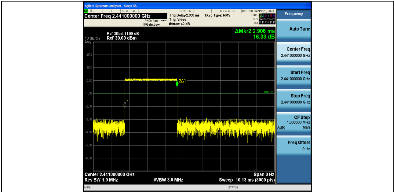
DH5-Ant1-Hop-PASS
