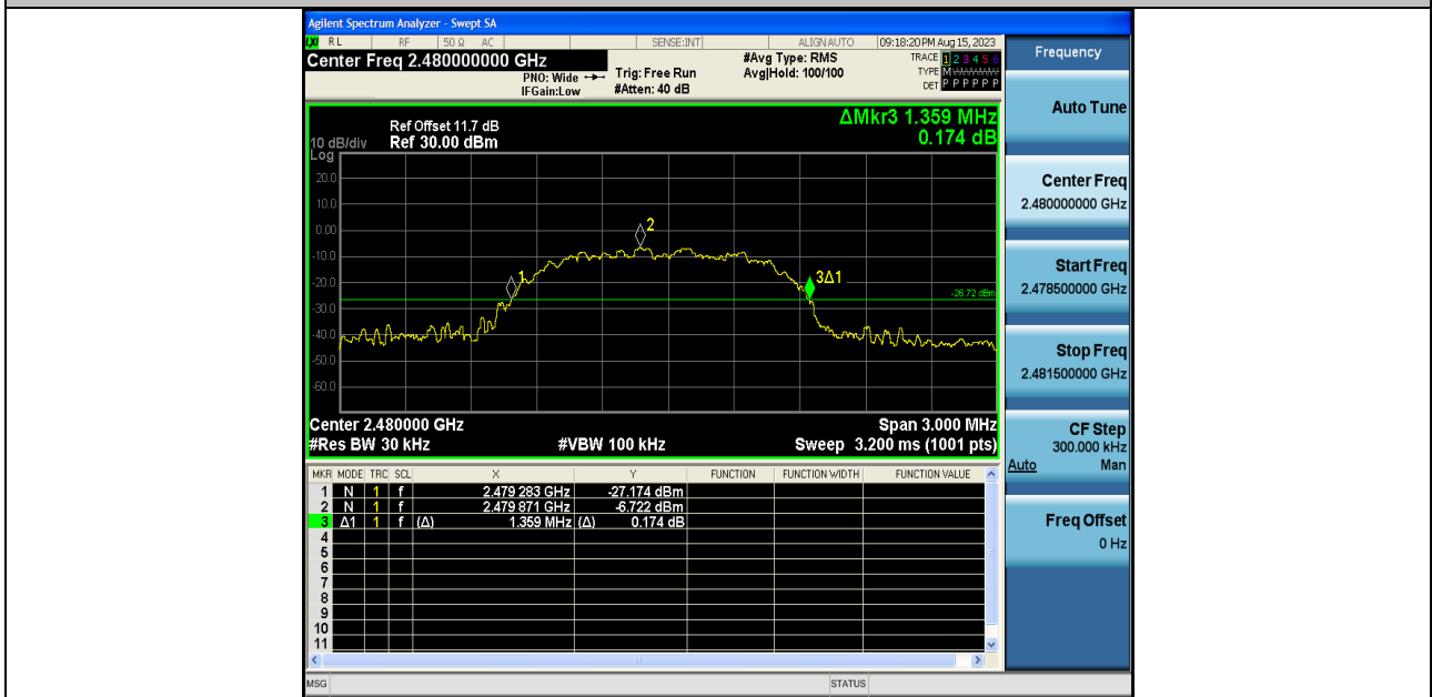
3DH5-Ant1-2480
