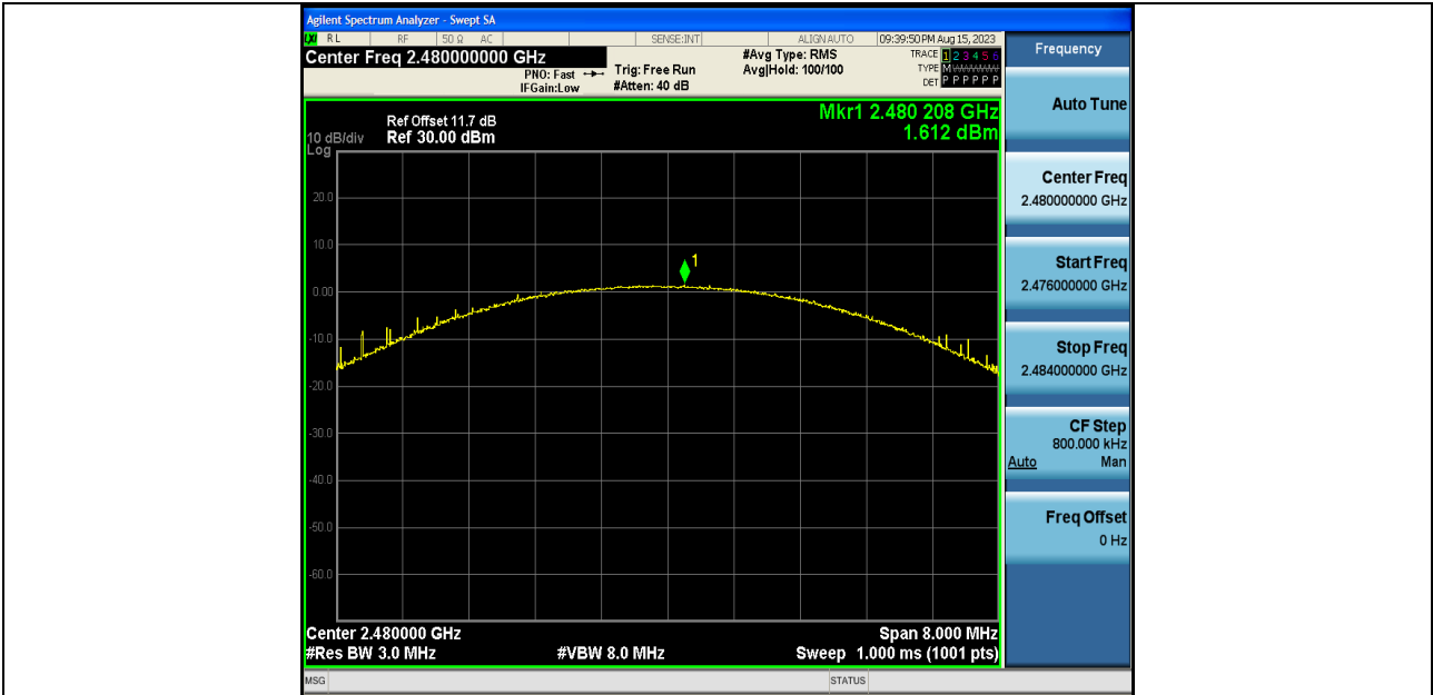
2DH5-Ant1-2480-PASS
