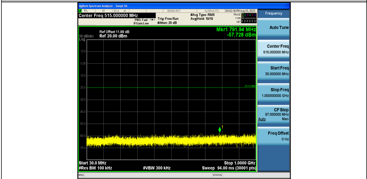
DH5-Ant1-2402-30~1000-PASS
