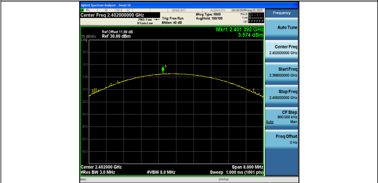
3DH5-Ant1-2402-PASS
