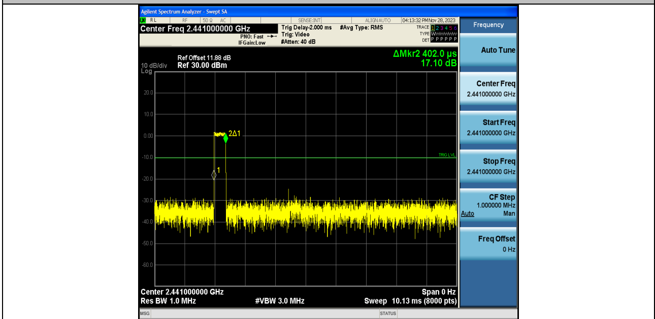
DH1-Ant1-Hop-PASS
