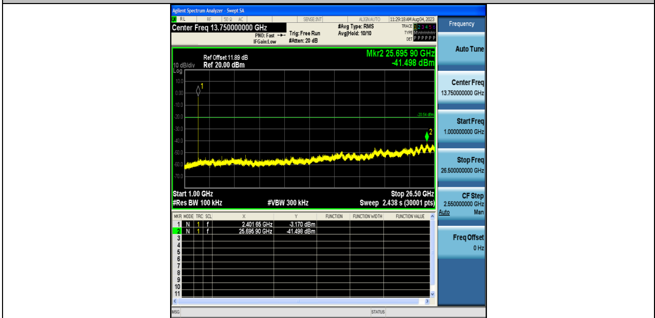
BLE_2M-Ant1-2402-1000~26500-PASS
