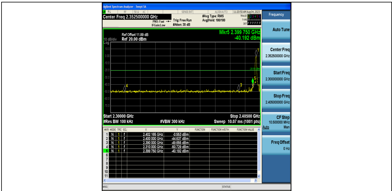
BLE_1M-Ant1-2402-PASS
