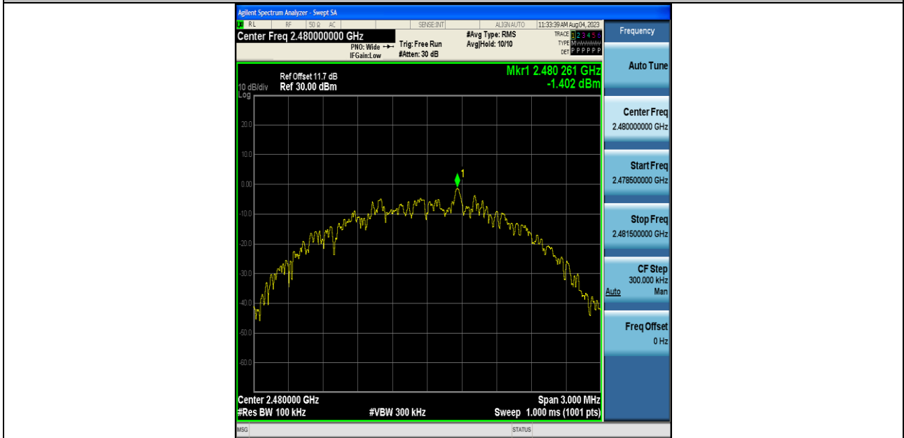
BLE_2M-Ant1-2480-0~Reference-PASS
