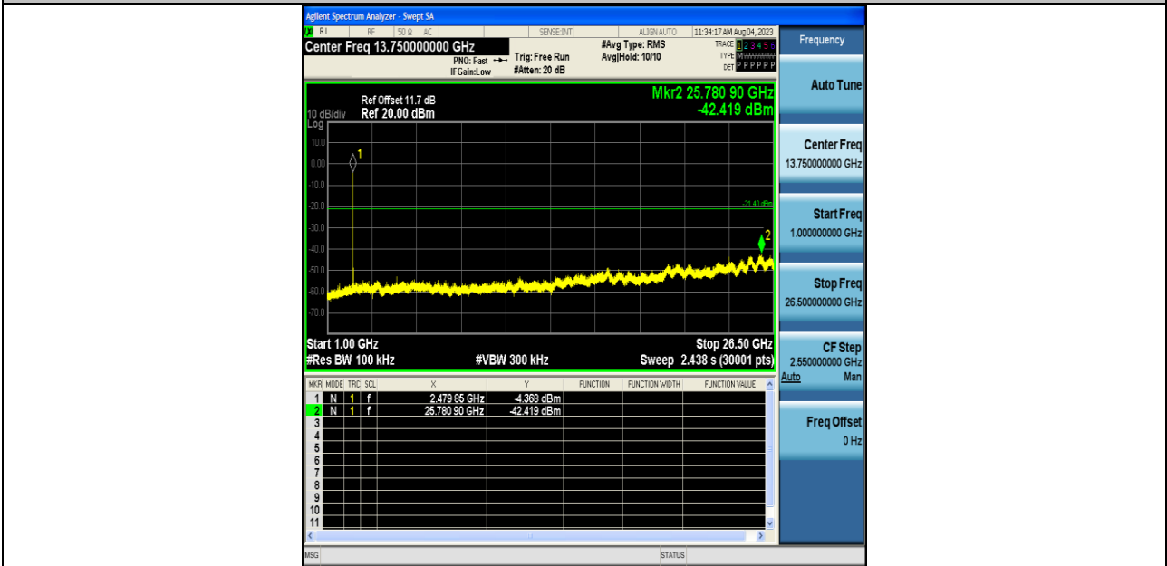
BLE_2M-Ant1-2480-1000~26500-PASS
