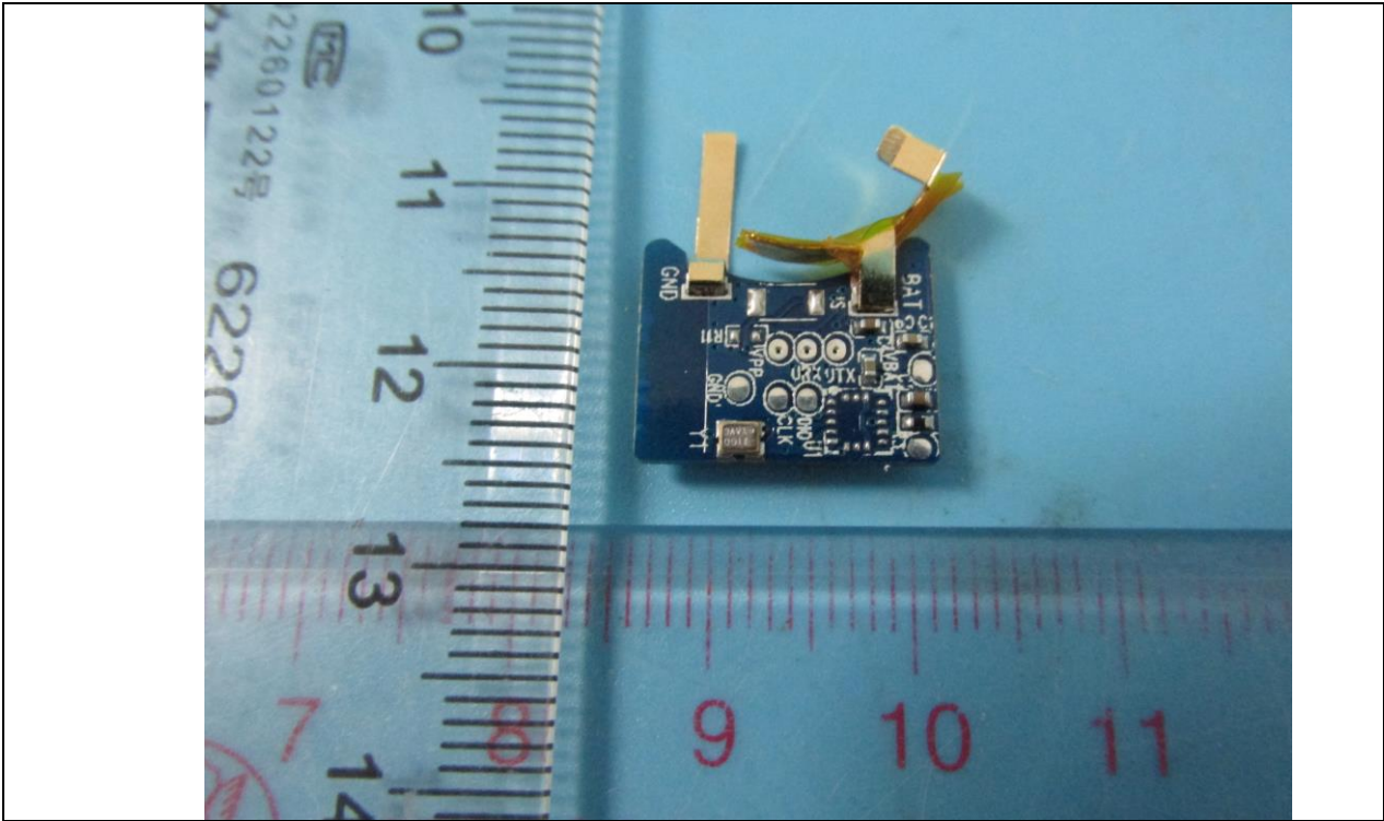
Details of: PCB view 1 (For model TWSD01A)
