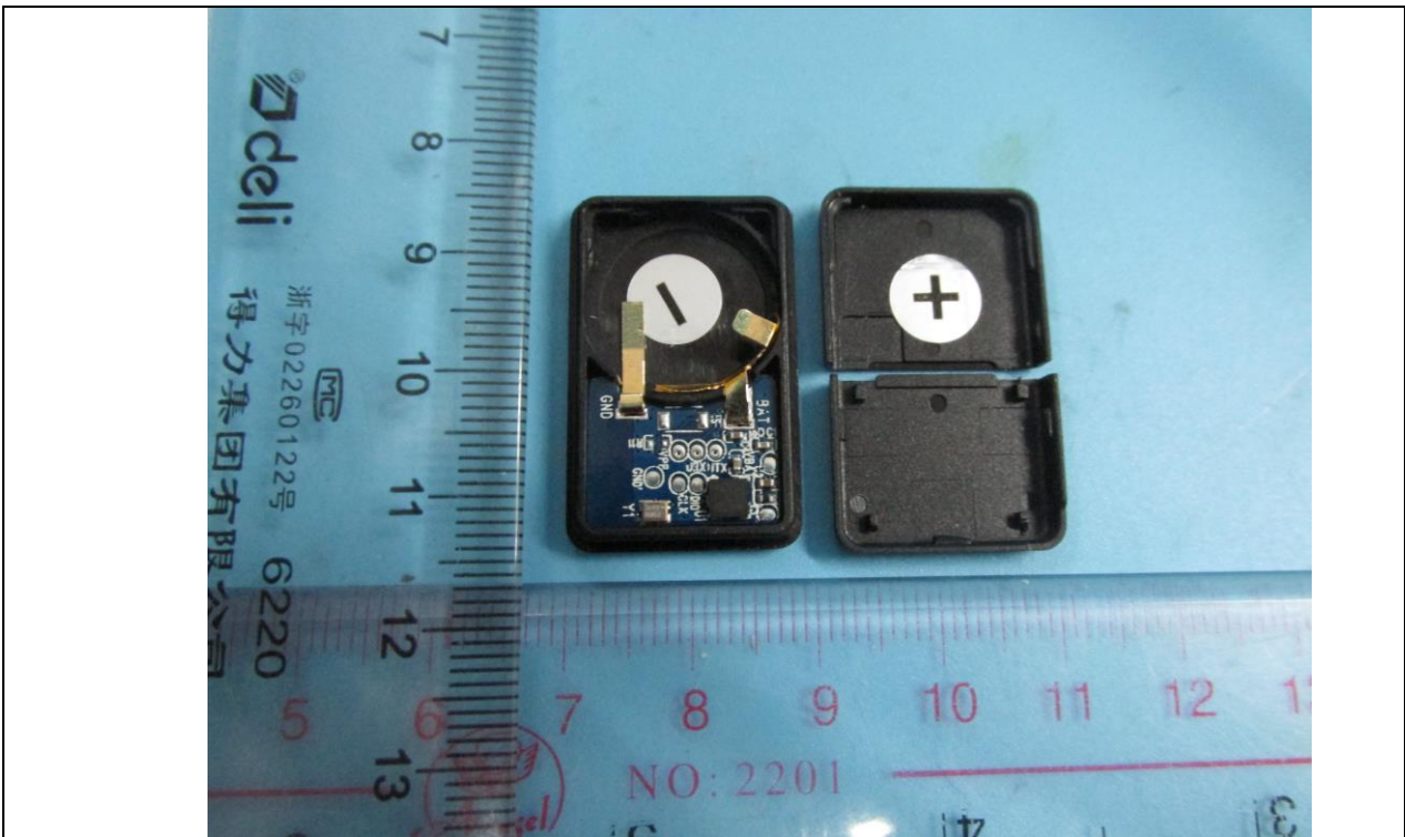
Details of: Internal view 2 (For model TBSD01A)
