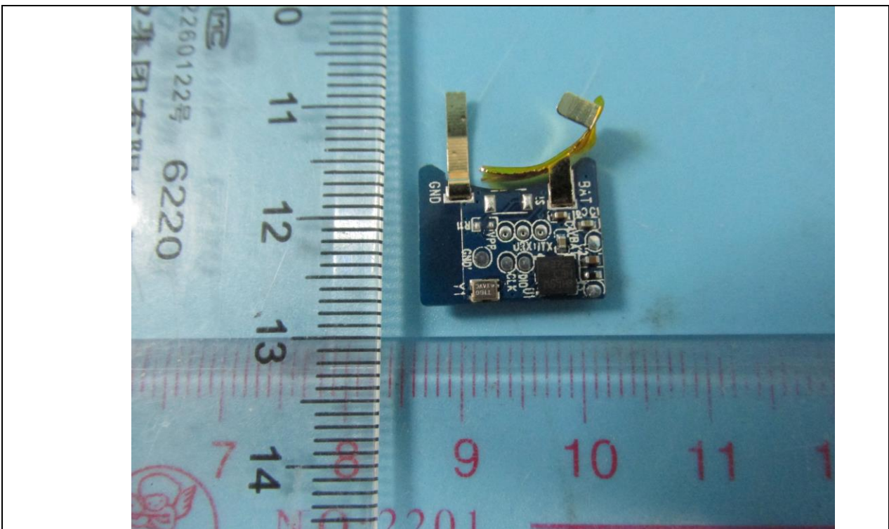
Details of: PCB view 2 (For model TBSD01A)
