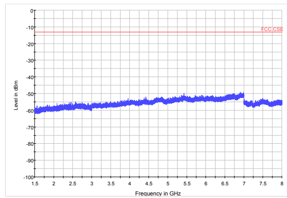
LTE Band 13 5MHz CH-High 1.5GHz~8GHz
