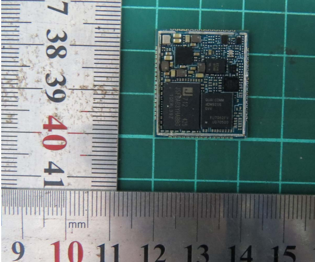
Picture 1 EUT and Accessory
