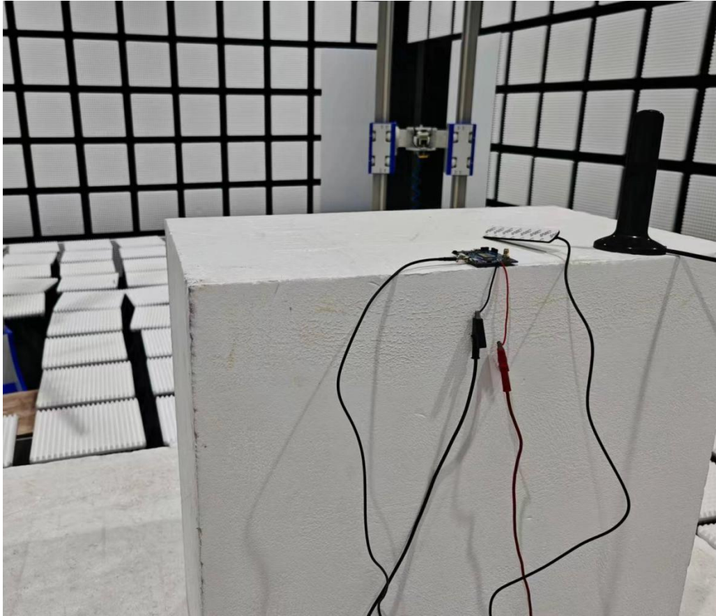
Pic2.RSE(Above 1GHz )
