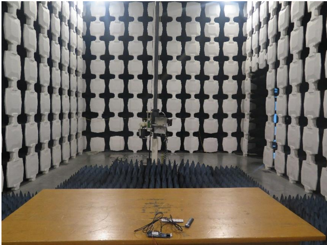
Pic2. Radiated emissions (1GHz-18GHz)
