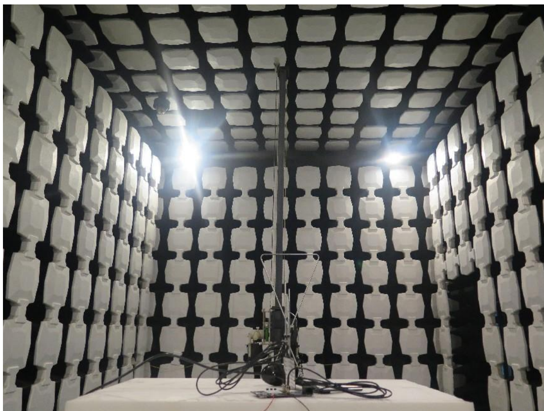
Pic3. Radiated spurious emission (30MHz-3GHz)
