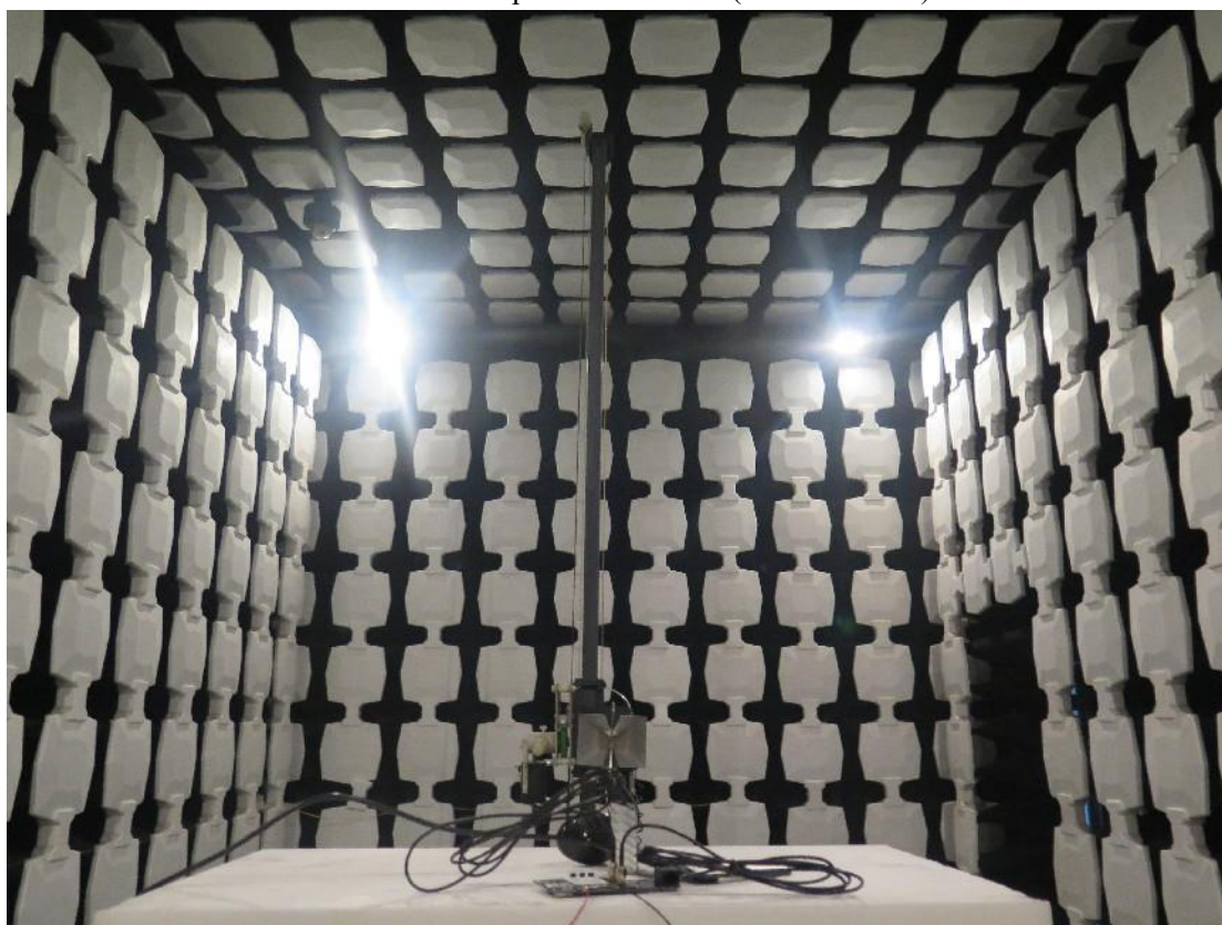
Pic4. Radiated spurious emission (3GHz-18GHz)
