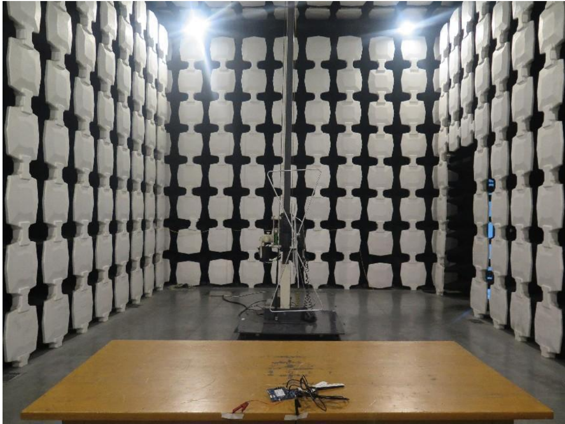
Pic1. Radiated emissions (30MHz-1GHz)
