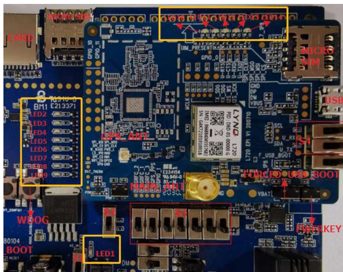
Figure5-9: Status indicator
