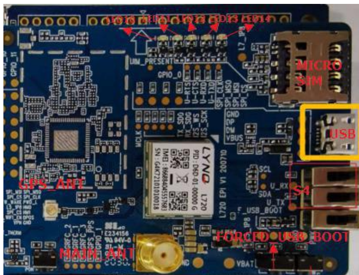
Figure5-4: USB 2.0 Port
