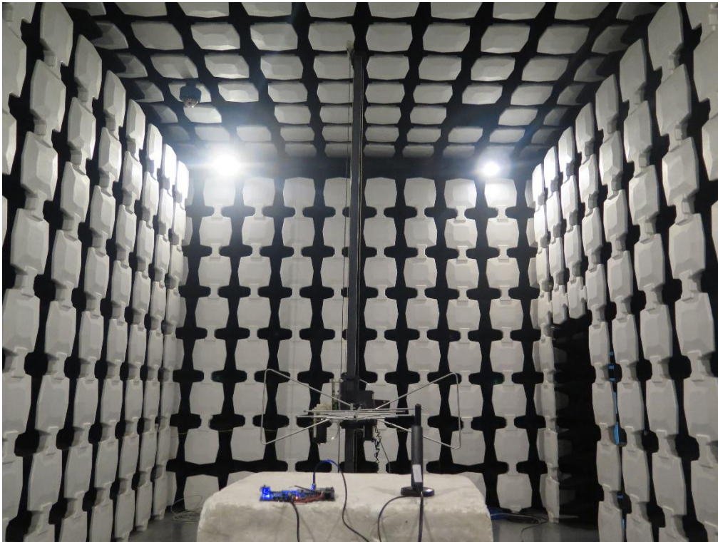
RSE (30MHz-3GHz)
