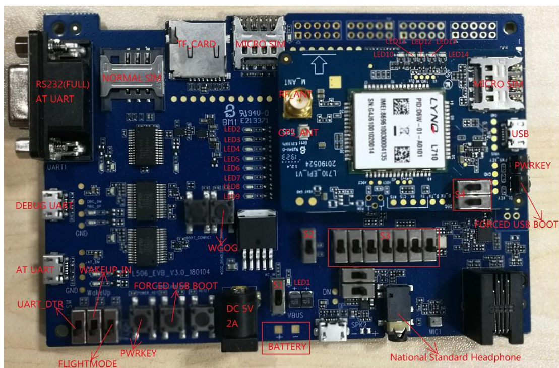
Figure 2-1: L710 EVB global graph
