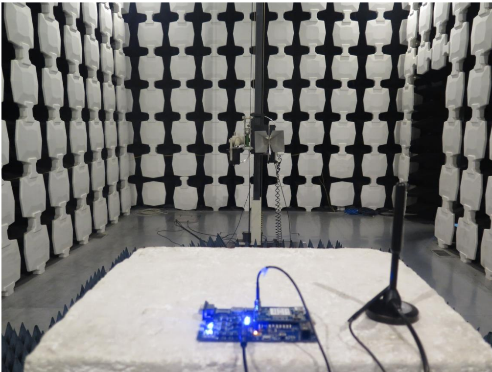
Pic4.RSE(3G-12.75G)
