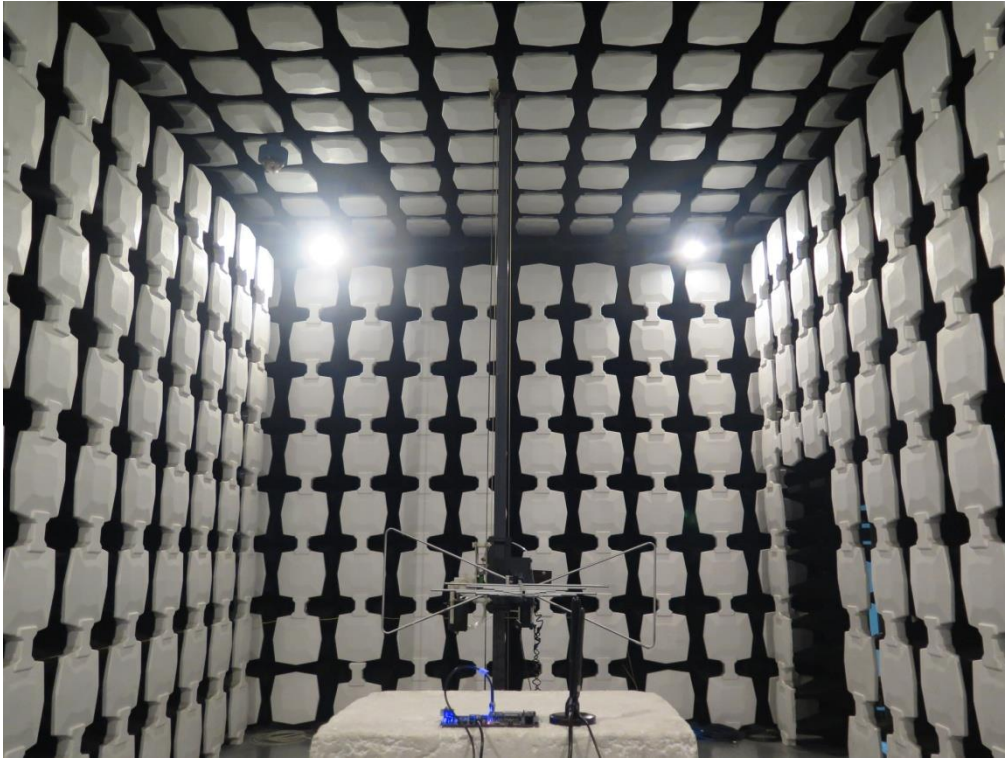
Pic3.RSE(30M-3G)
