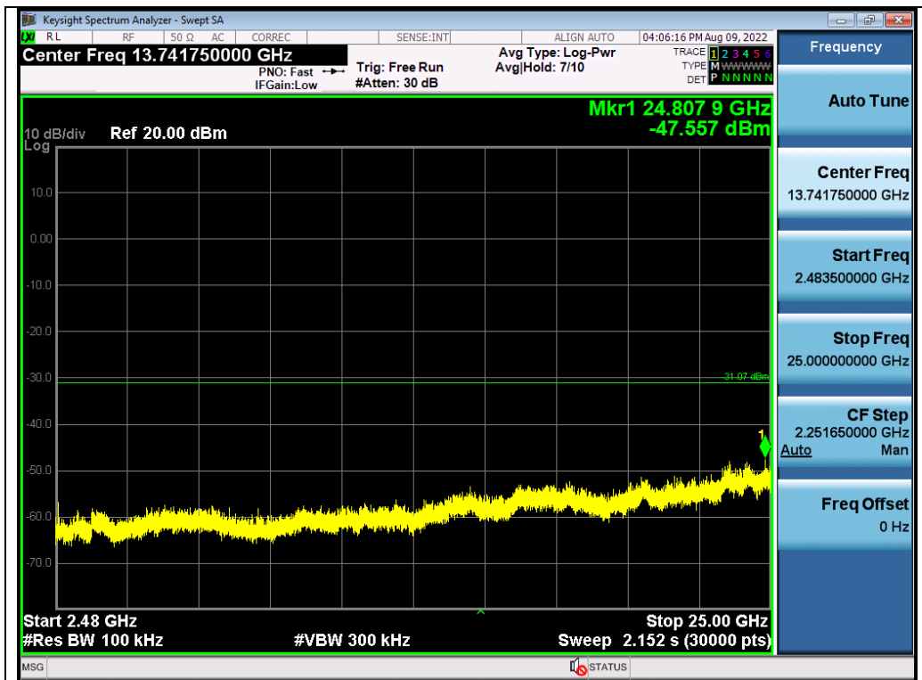
Test_Graph_FSK_ANT1_2408_2Mbps_Higher Band Emissions
