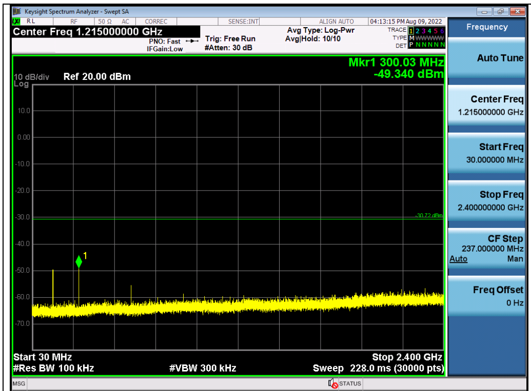
Test_Graph_FSK_ANT1_2440_2Mbps_Lower Band Emissions
