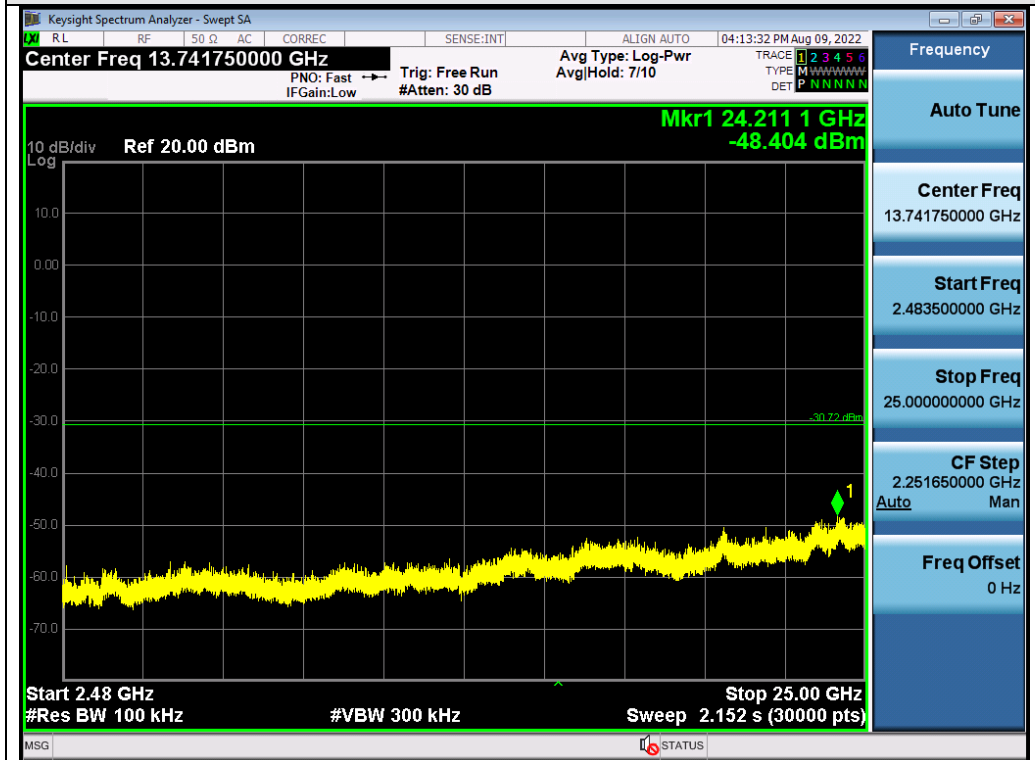
Test_Graph_FSK_ANT1_2440_2Mbps_Higher Band Emissions
