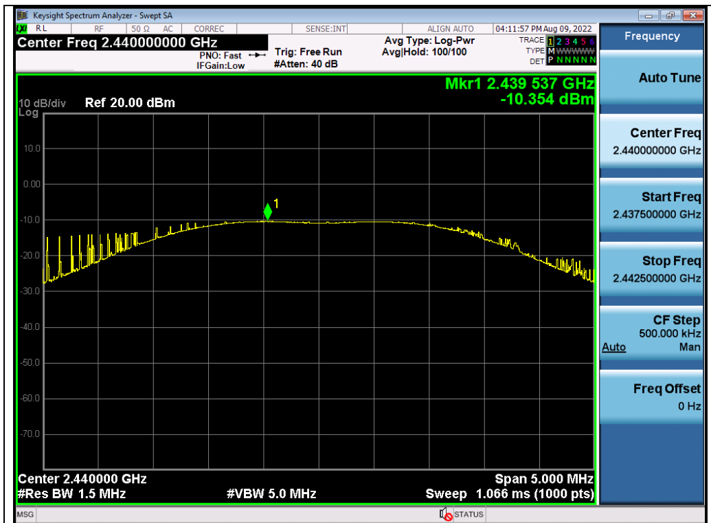
Test_Graph_FSK_ANT1_2440_2Mbps_Peak Power
