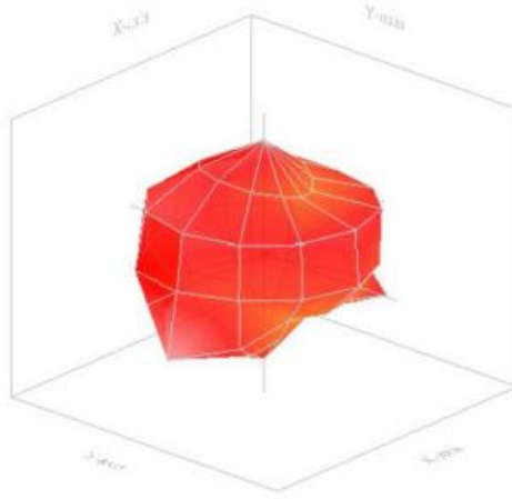
Radiation pattern
