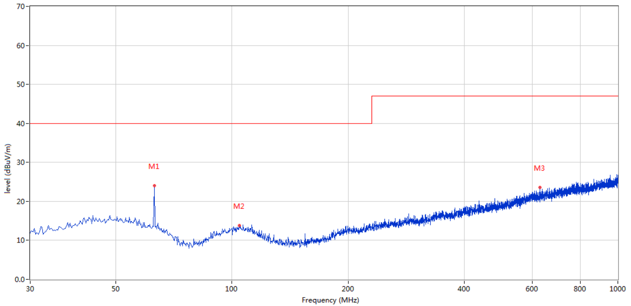
CE_EN 55032 Class B 30MHz-1GHz
