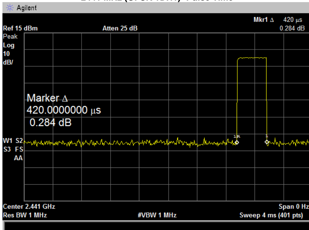
2441 MHz (GFSK 1DH1)- Pulse Time
