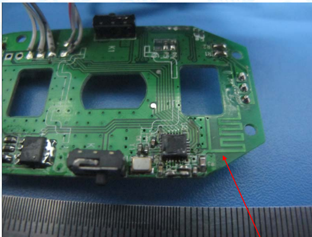
2.4G PCB Antenna
