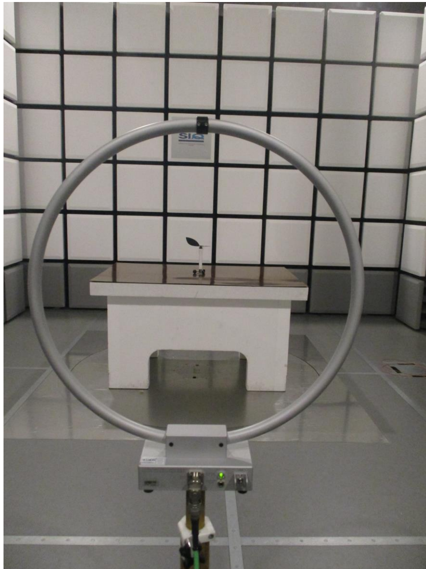
Figure 1: Radiated emission test, 9 kHz – 30 MHz
