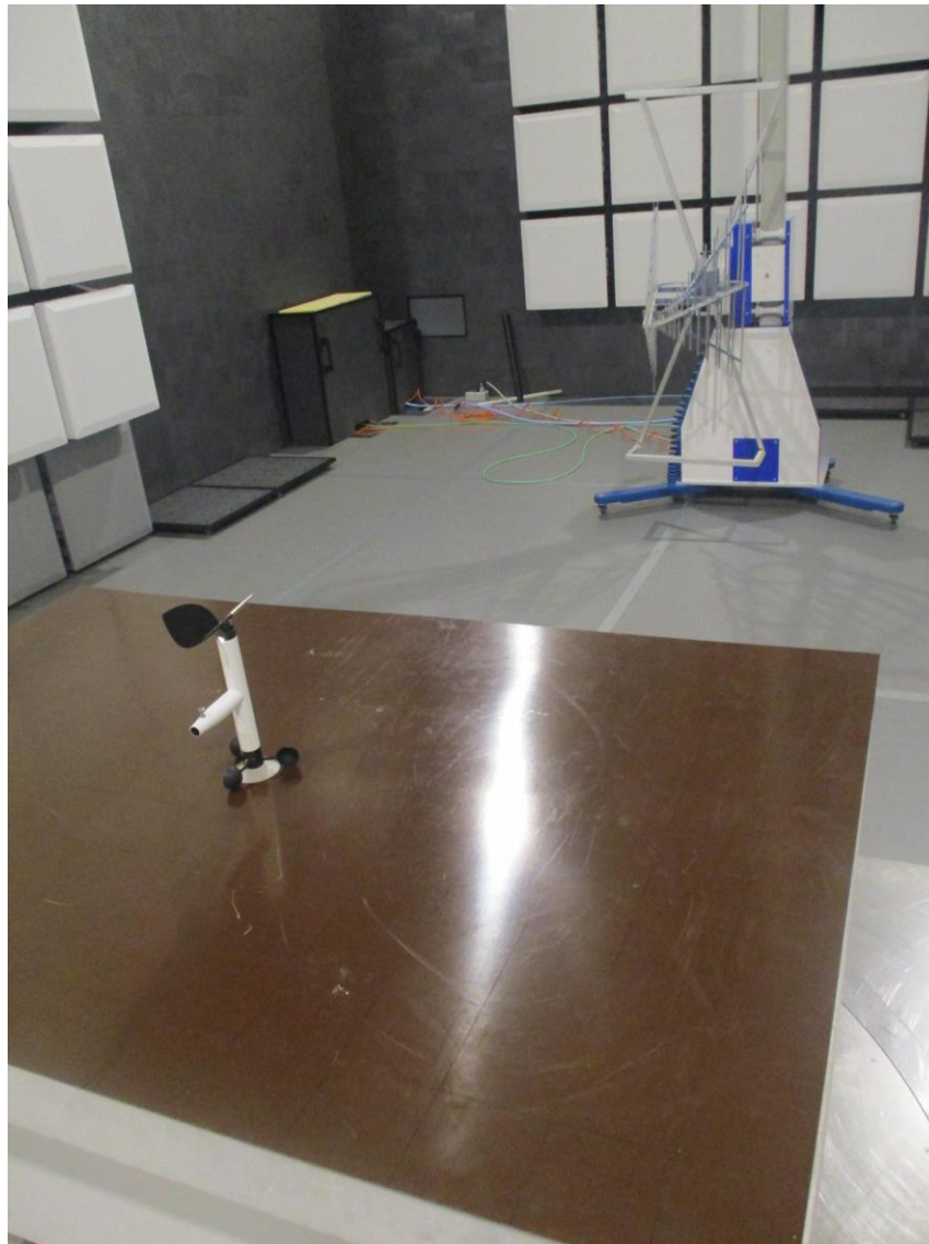
Figure 3: Radiated emission test, 200 MHz – 1 GHz
