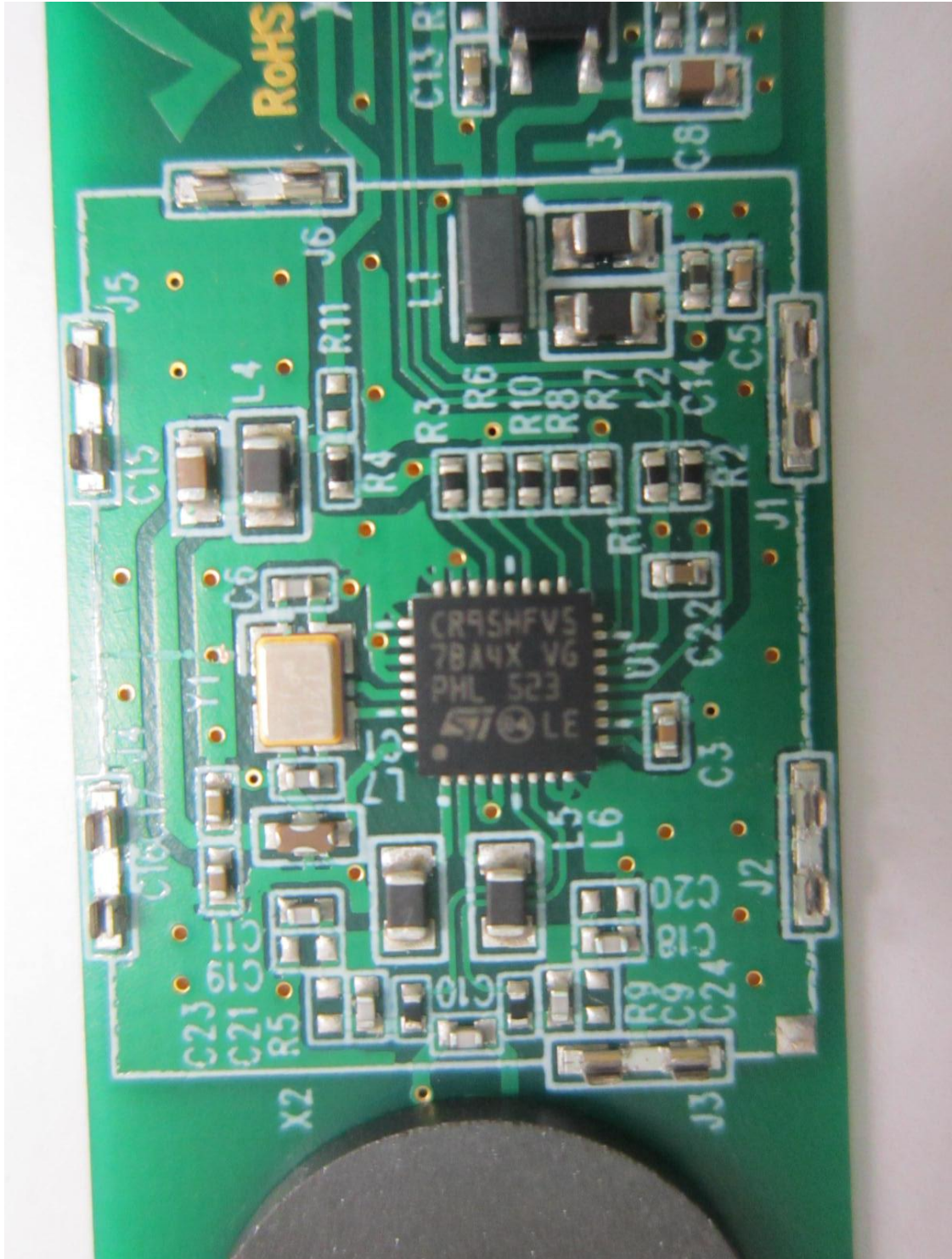
RF Module Circuit with RF Shield Removed (Close-up)
