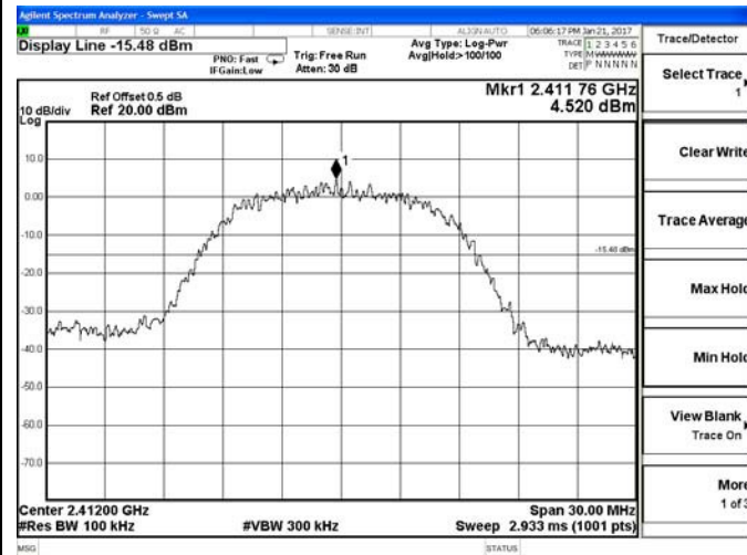
Channel 1 / 2412 MHz
