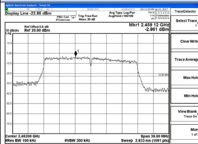
Channel 11 / 2462 MHz
