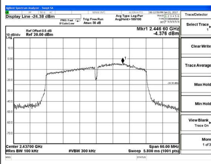
2407 – 2467 MHz
