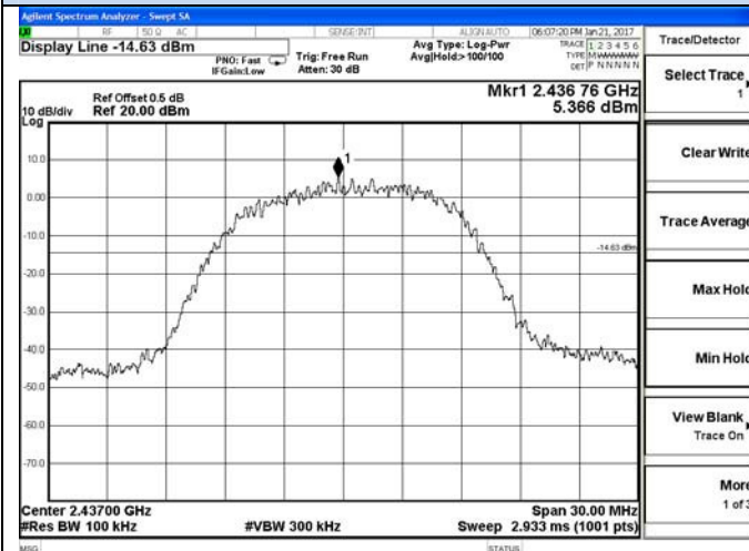
2422 – 2452 MHz
