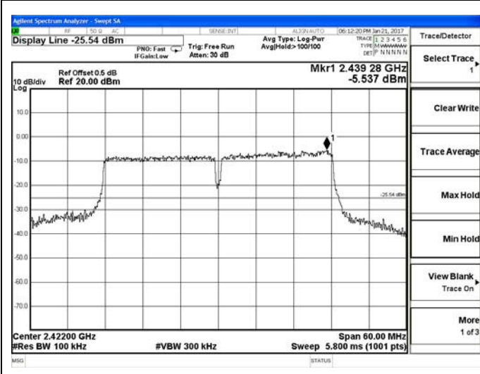
2392 – 2452 MHz
