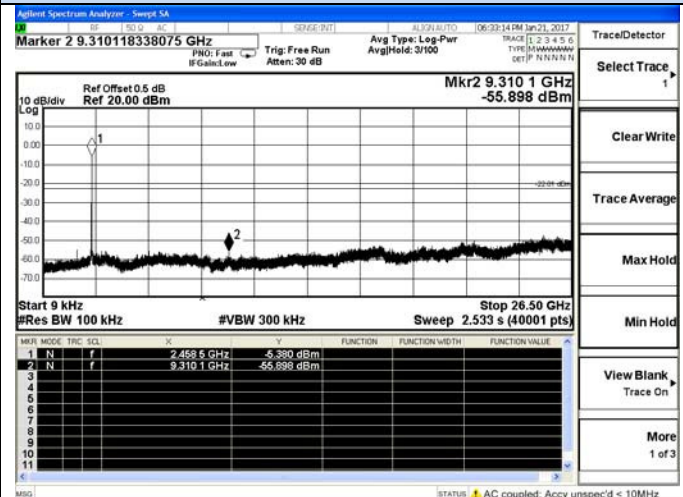
9 KHz – 26.5 GHz
