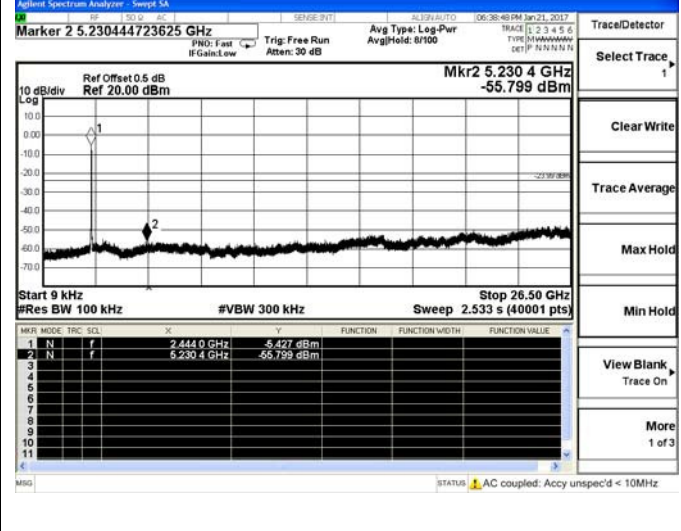
9 KHz – 26.5 GHz
