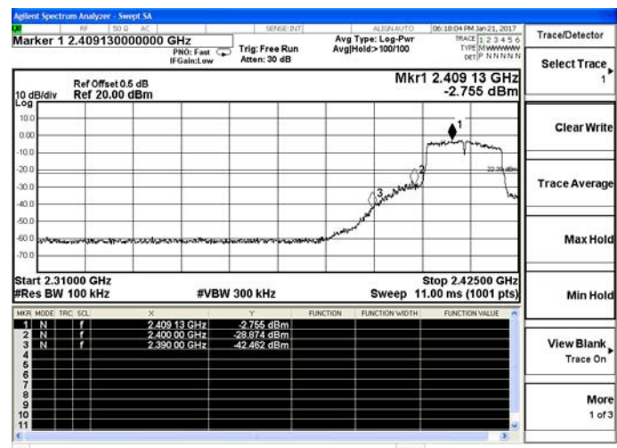
Channel 1 / 2412 MHz
