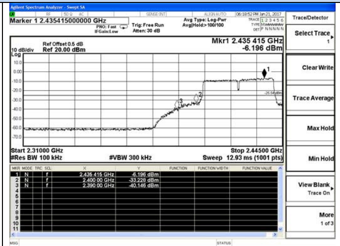
Channel 3 / 2422 MHz
