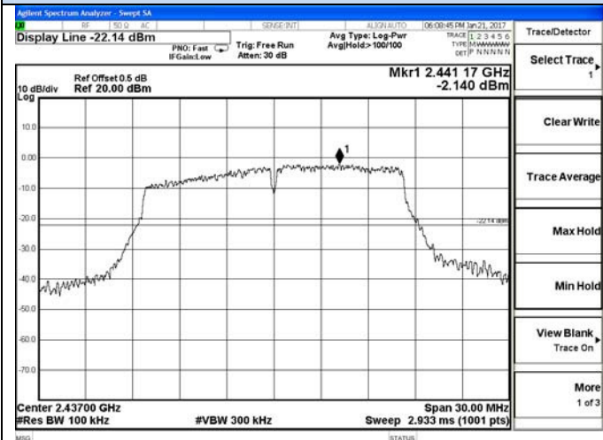
2422 – 2452 MHz
