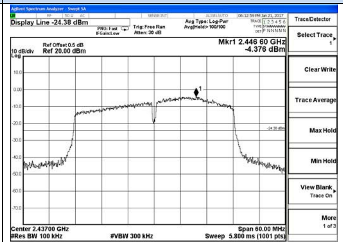
Channel 6 / 2437 MHz
