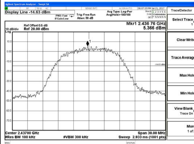
Channel 6 / 2437 MHz
