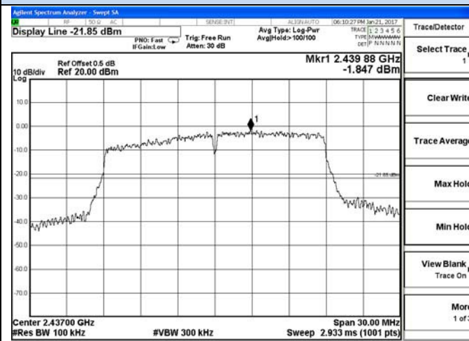
Channel 6 / 2437 MHz
