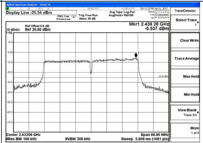
Channel 3 / 2422 MHz
