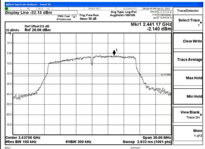
Channel 6 / 2437 MHz
