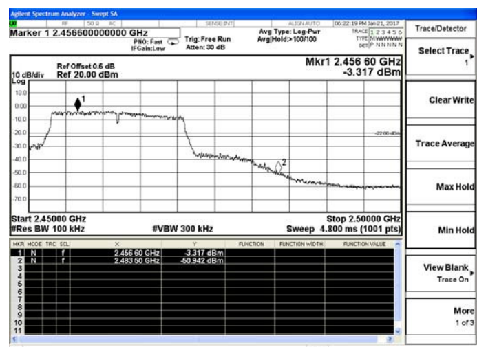
Channel 11 / 2462 MHz
