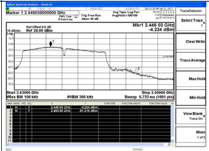
Channel 9 / 2452 MHz
