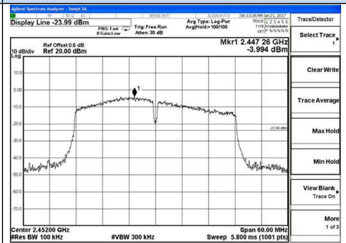
Channel 9 / 2452 MHz
