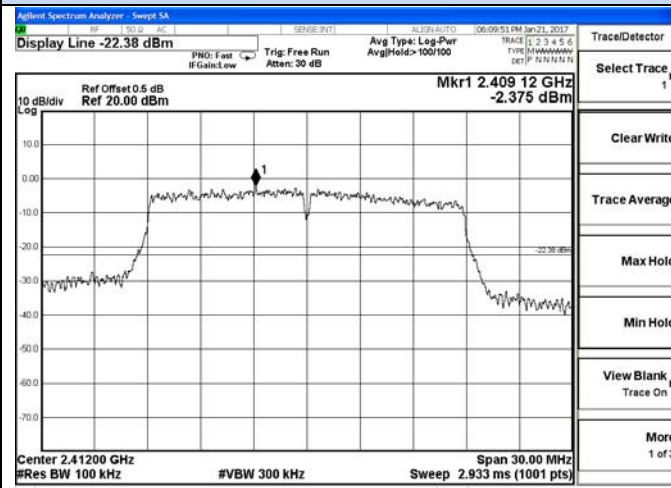
Channel 1 / 2412 MHz
