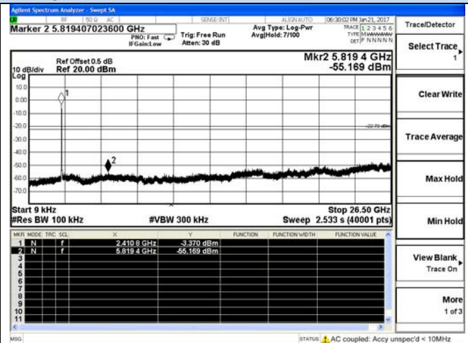
9 KHz – 26.5 GHz
