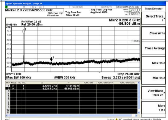
9 KHz – 26.5 GHz
