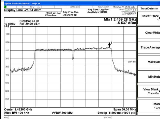
2392 – 2452 MHz
