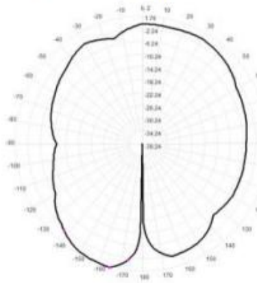
915MHZ, Total=YZ, Max=1.5dBi
