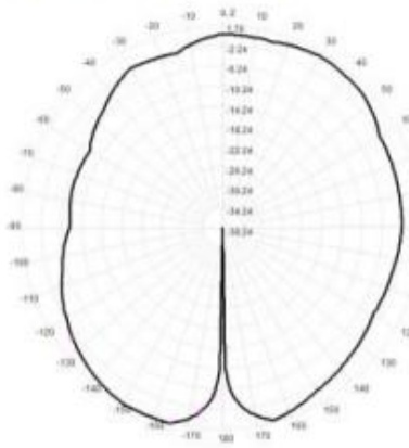
915MHZ, Total=XZ, Max=1.5dBi
