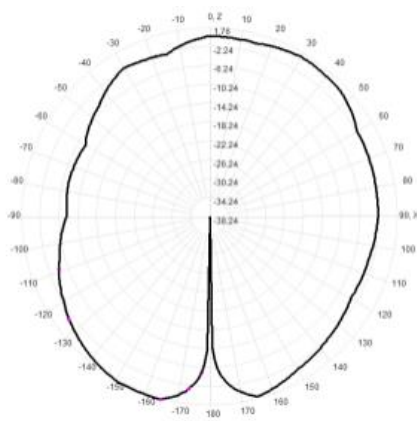
915MHZ, Total=XZ, Max=1.5dBi
