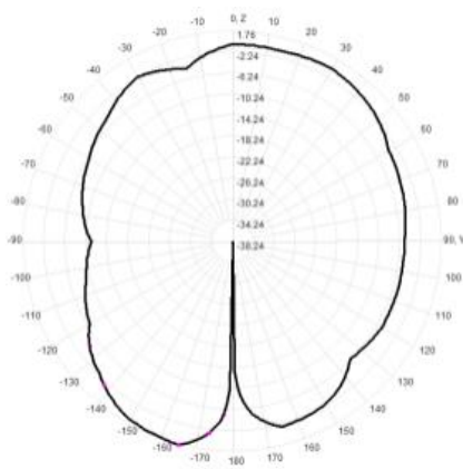
915MHZ, Total=YZ, Max=1.5dBi
