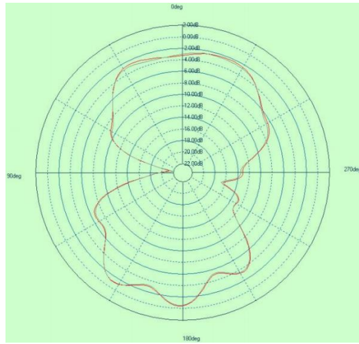
Phi=0°
