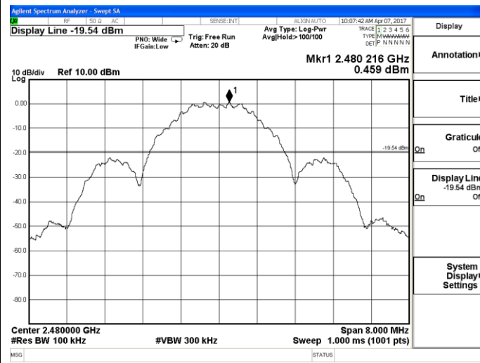
Channel 16 / 2480 MHz
