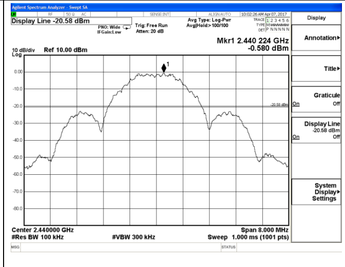
Channel 8 / 2440 MHz
