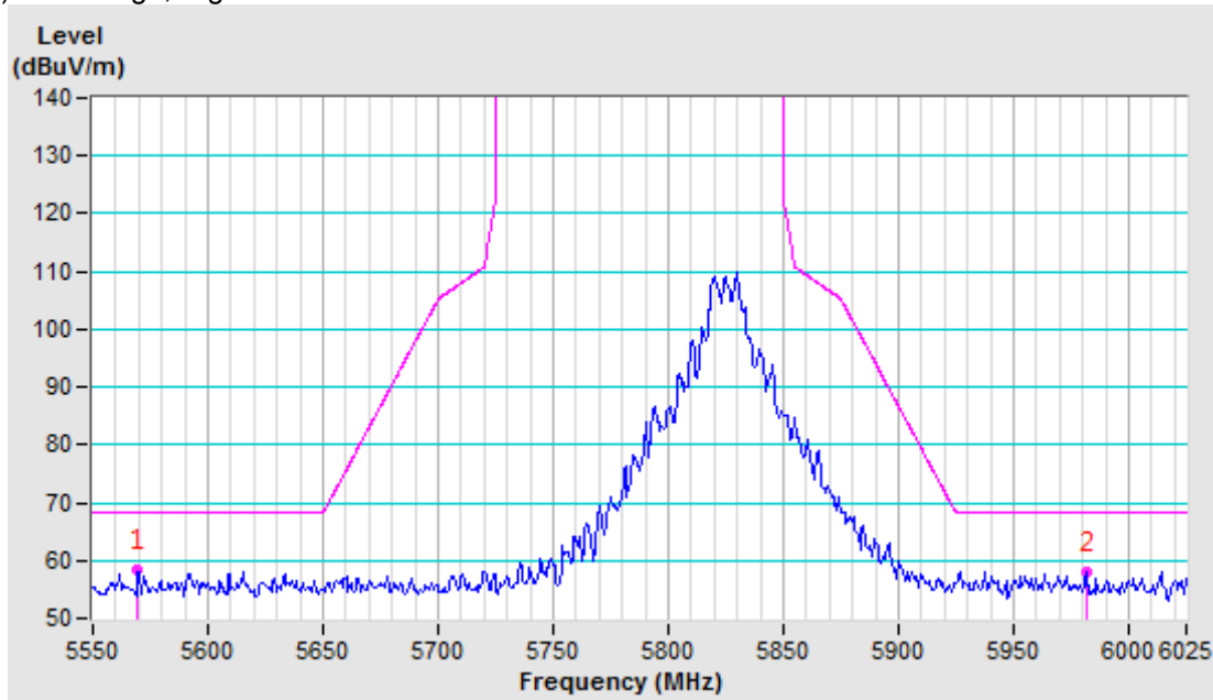
(802.11a) Band Edge, Right Side
