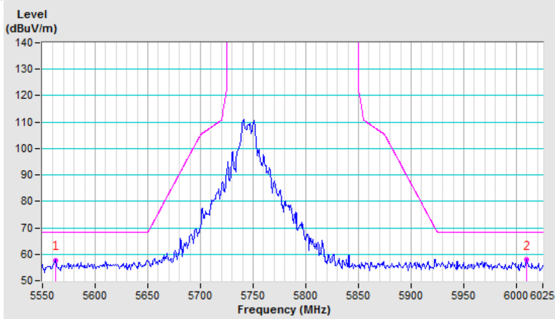
(802.11a) Band Edge, Left Side
