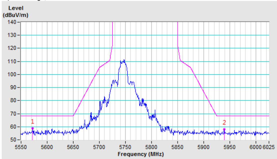
(802.11n20) Band Edge, Right Side
