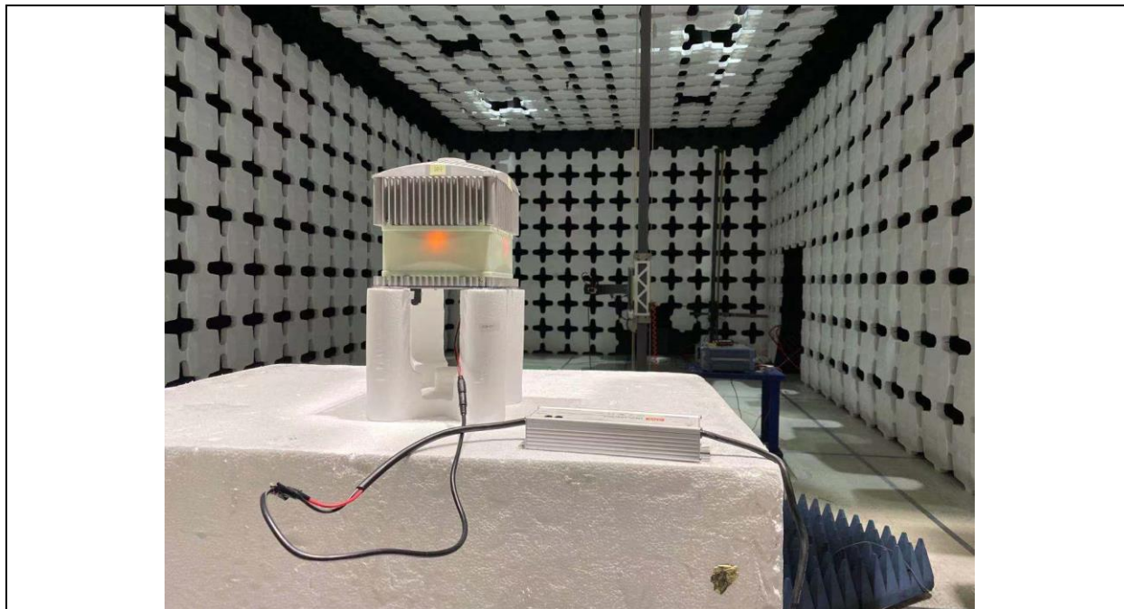
Radiated Emission Test above 40GHz Rear View
