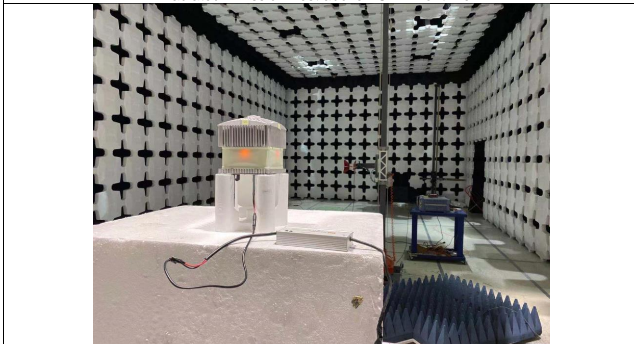
Radiated Emission Test above 1GHz Rear View
