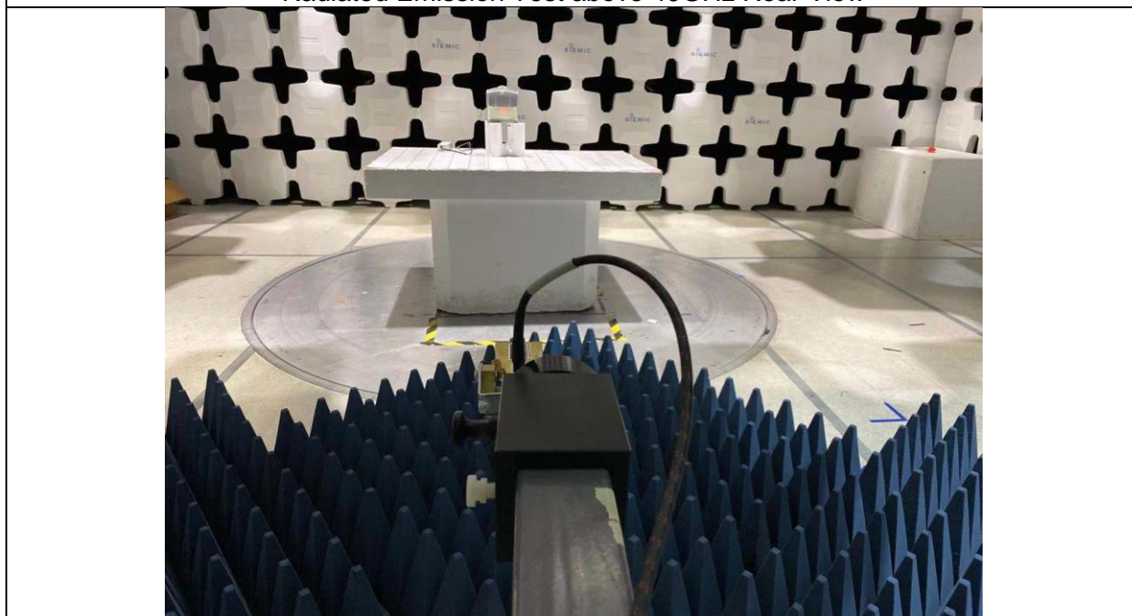
Radiated Emission Test above 40GHz Front View
