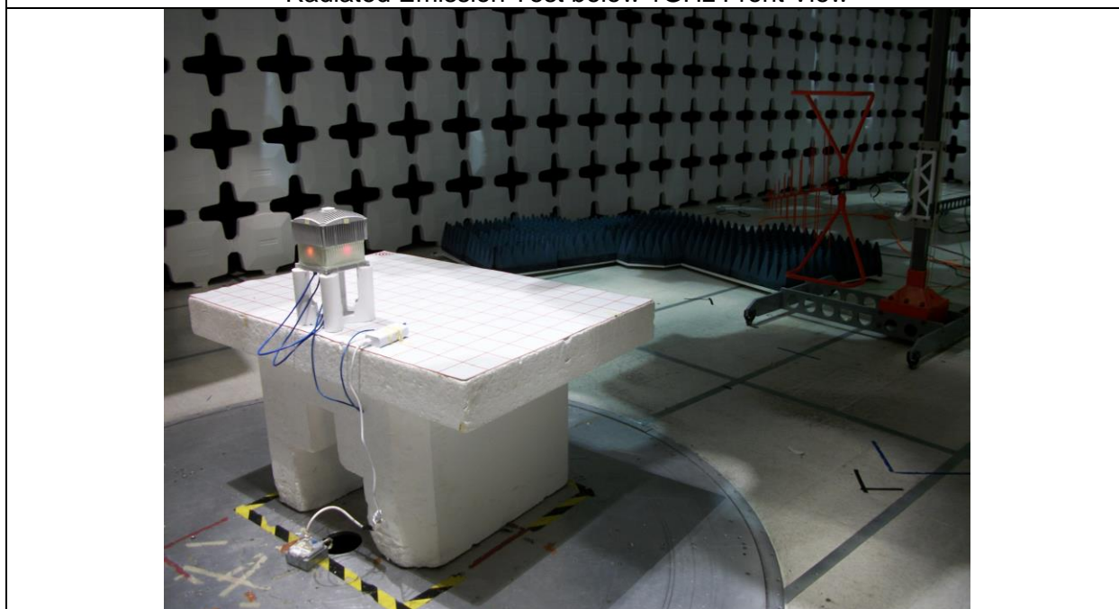
Radiated Emission Test below 1GHz Rear View
