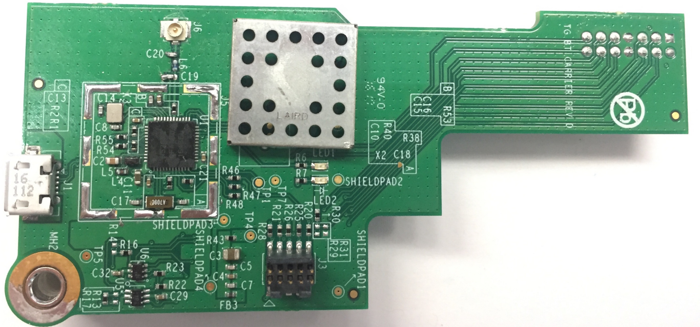
Top side without the shield cover
