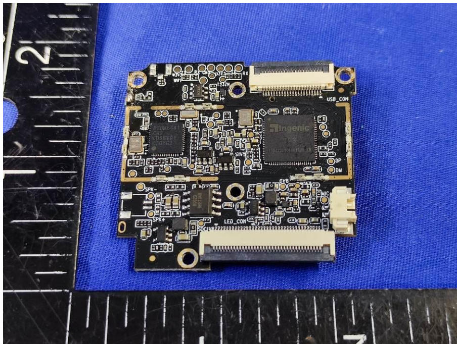
TVD100 series
