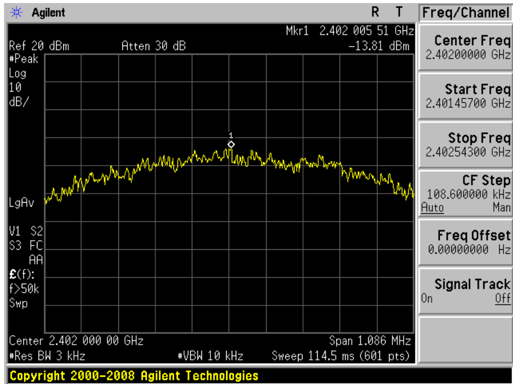
Power spectral density plot on channel 00 1Mbps
