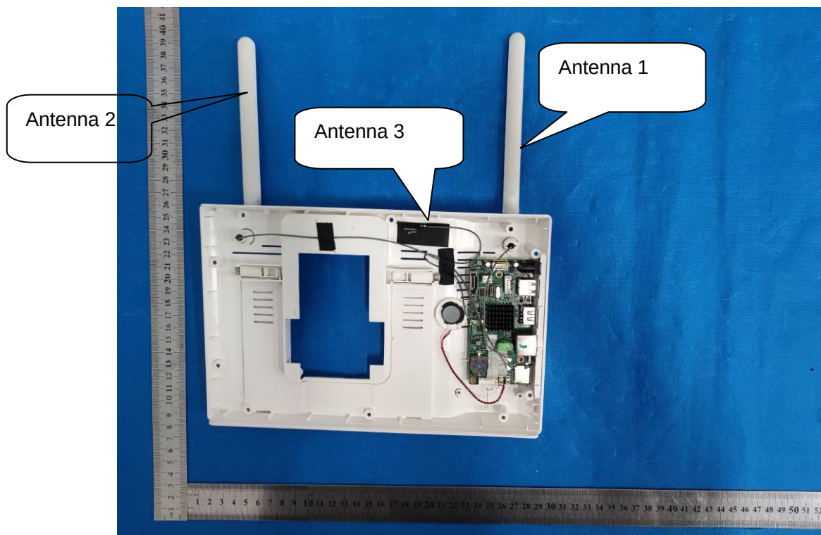
ANTENNA CLOSE-UP PHOTO-1
