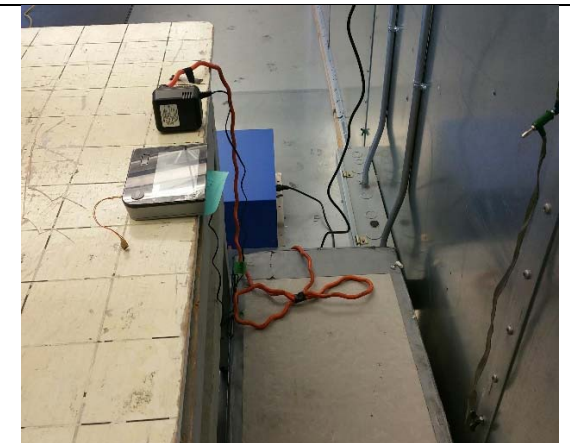
Conducted AC Mains Measurements
