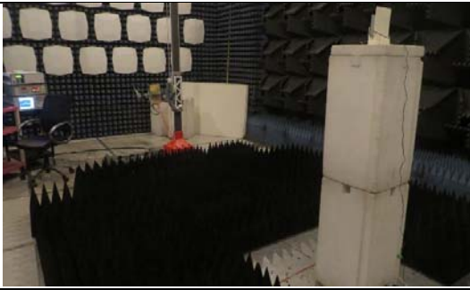
> 1 GHz Tx
