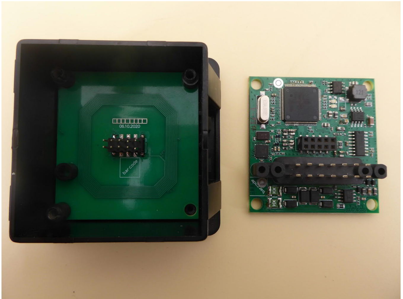
EUT, main PCB removed
