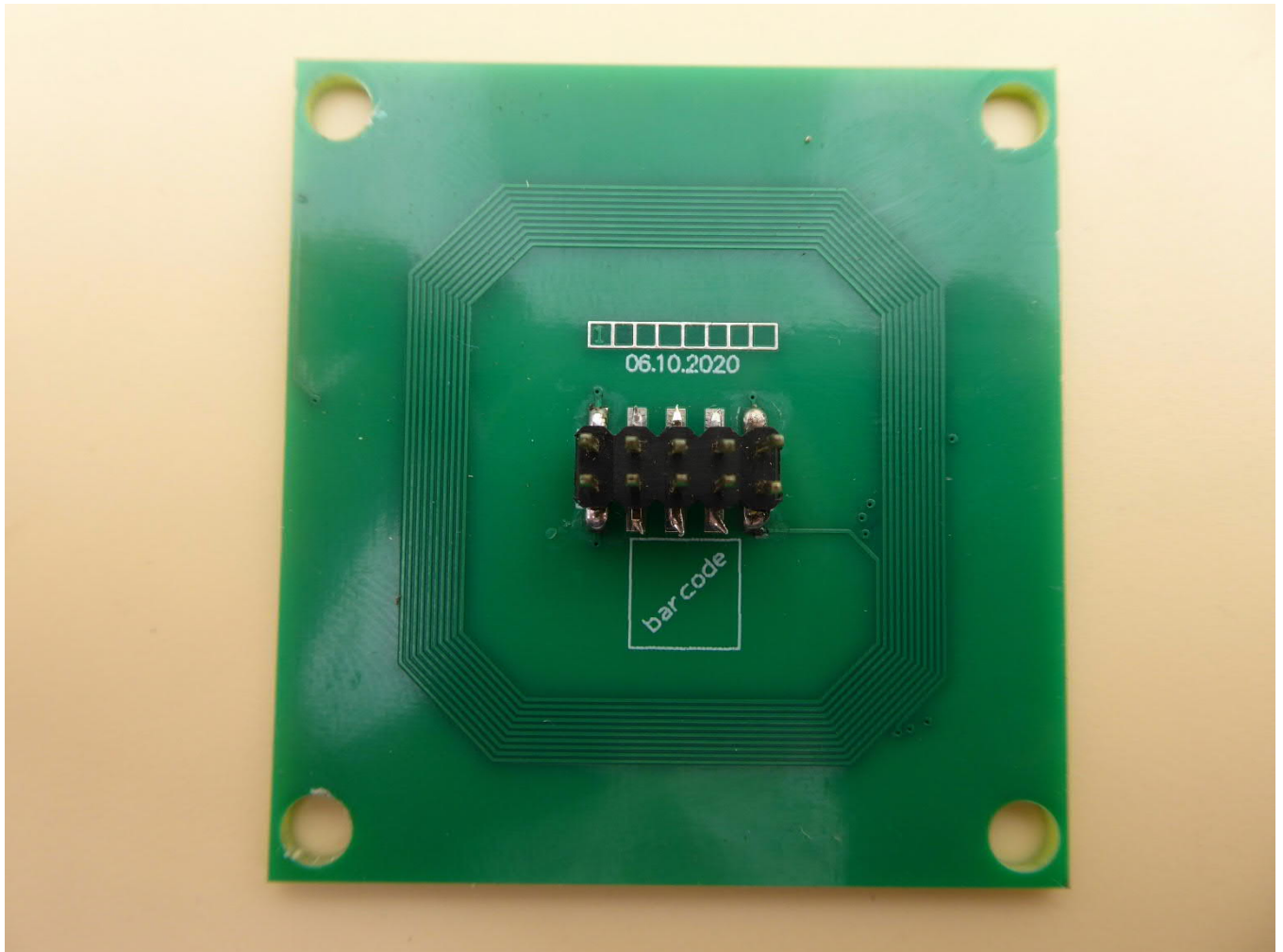
Antenna PCB, top view
