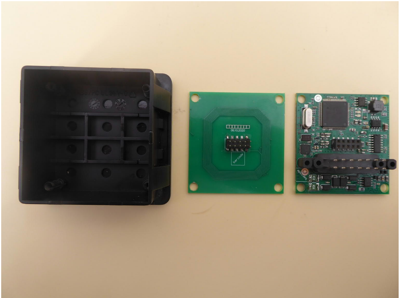
EUT, main and antenna PCB removed
