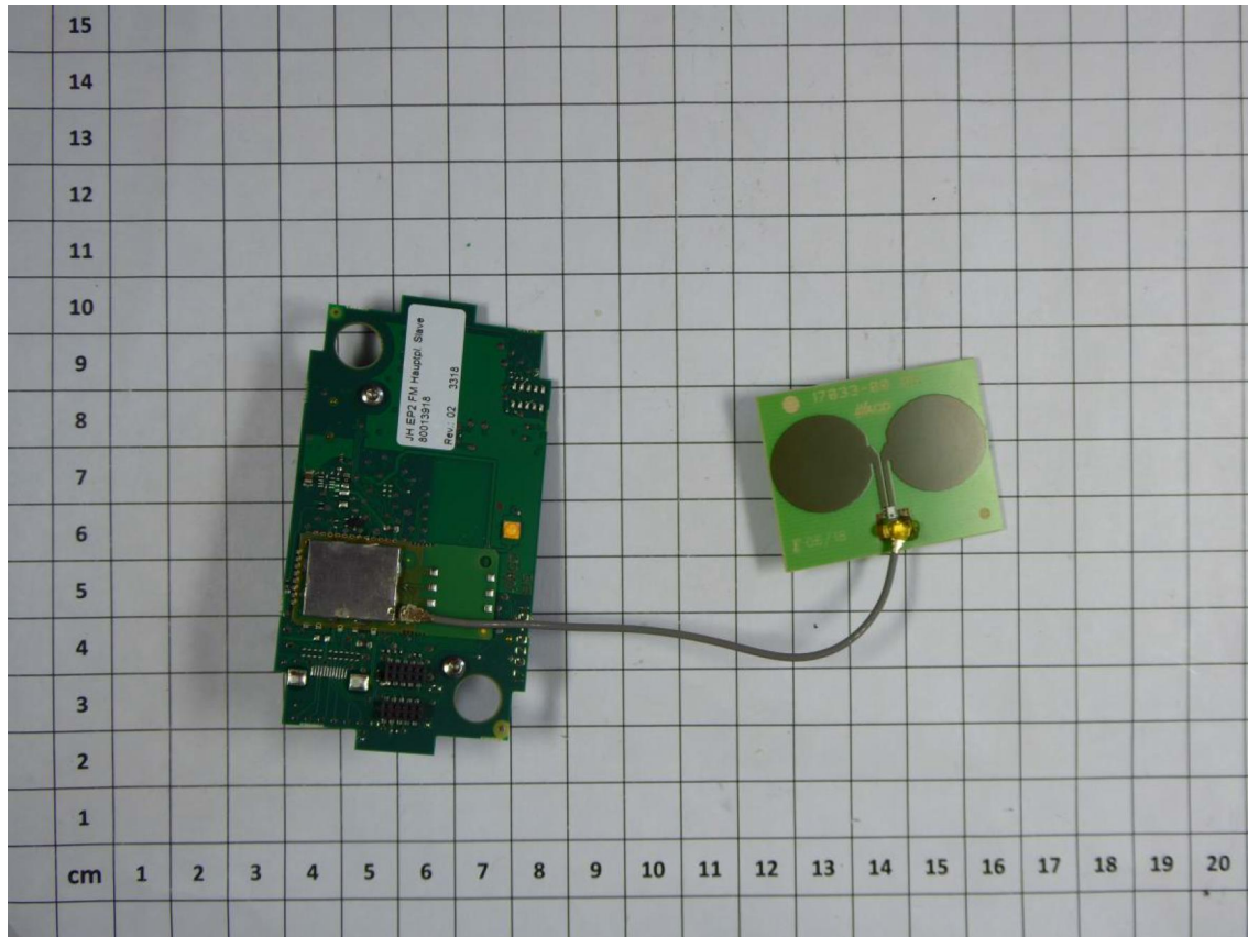
UWB board without screening shield
