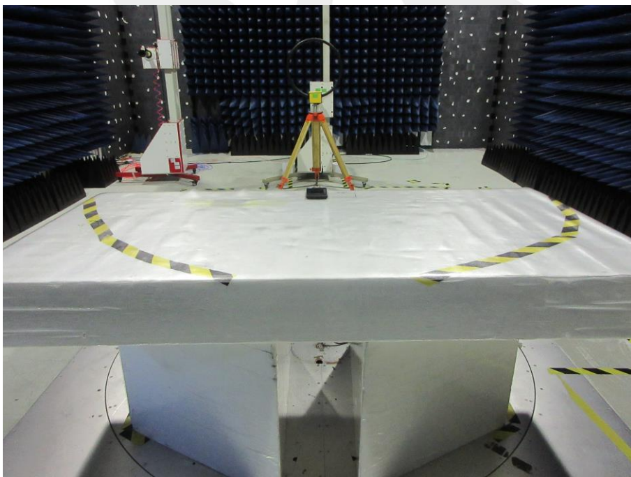
DXX radiation 9K-30MHz
