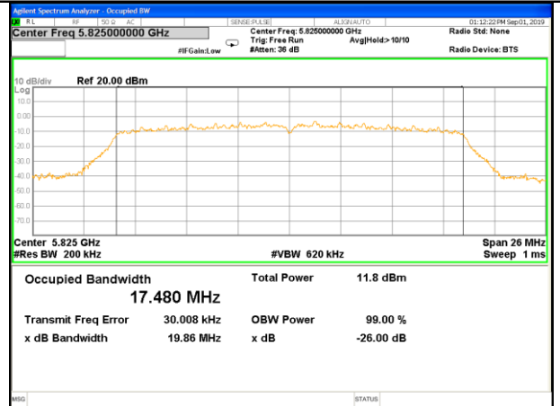
W58_11n20_Higher_26BW and 99%
