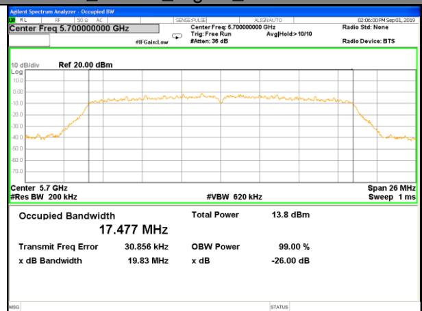
W56_11ac20_Higher_26BW and 99%
