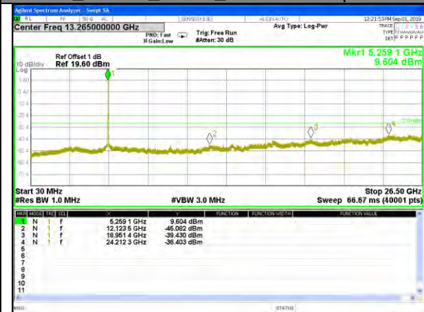
W53_11ac20_Higher_Conducted Spurious
