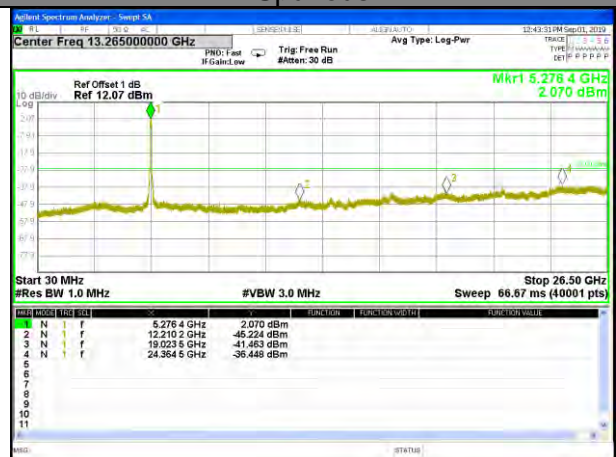
W53_11ac80_CH58(5290MHz)_Conducted Spurious
