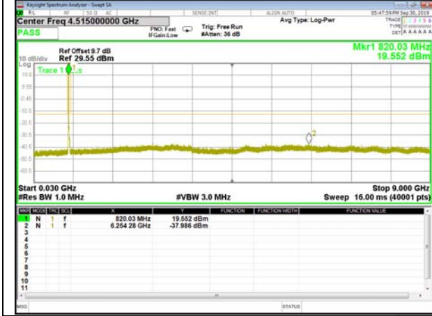
B26_QPSK_10M_Low_CDT_Spurious
