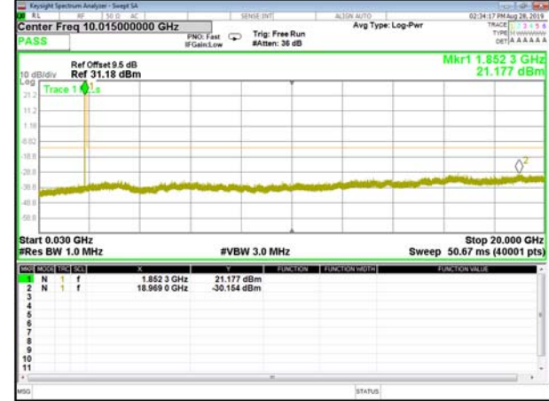
B25_QPSK_3M_Mid_CDT_Spurious
