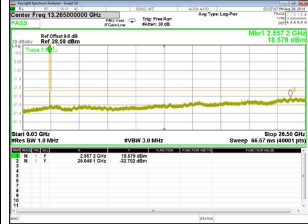
B41_QPSK_5M_Mid_CDT_Spurious
