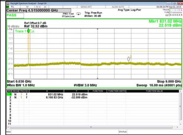
B26_QPSK_3M_High_CDT_Spurious
