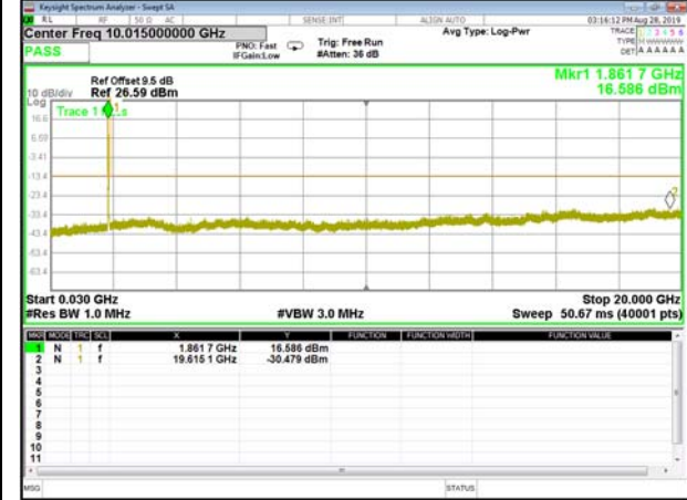
B25_QPSK_20M_Mid_CDT_Spurious
