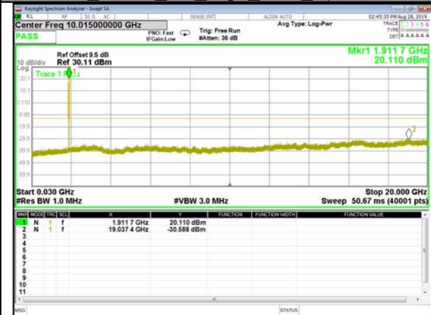
B25_QPSK_5M_High_CDT_Spurious
