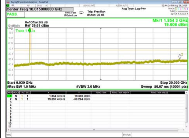
B25_QPSK_5M_Mid_CDT_Spurious
