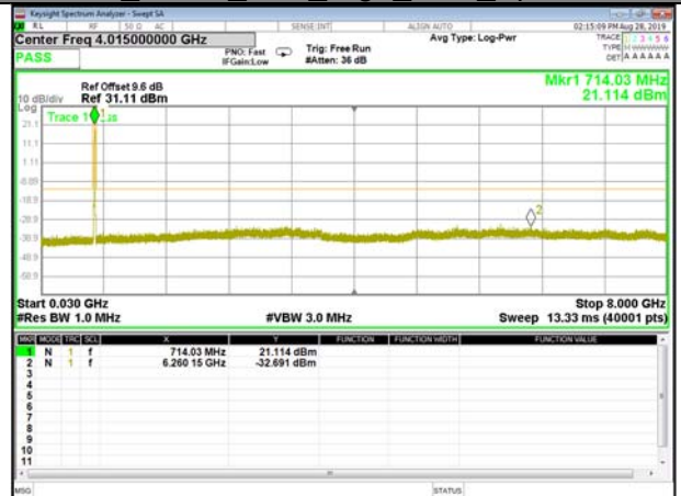
B17_QPSK_10M_High_CDT_Spurious
