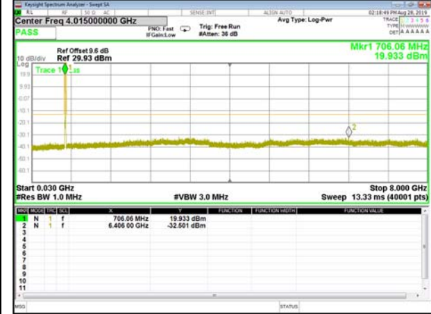
B17_Q16_10M_Mid_CDT_Spurious
