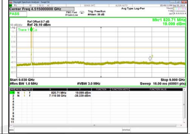
B26_Q16_10M_Low_CDT_Spurious
