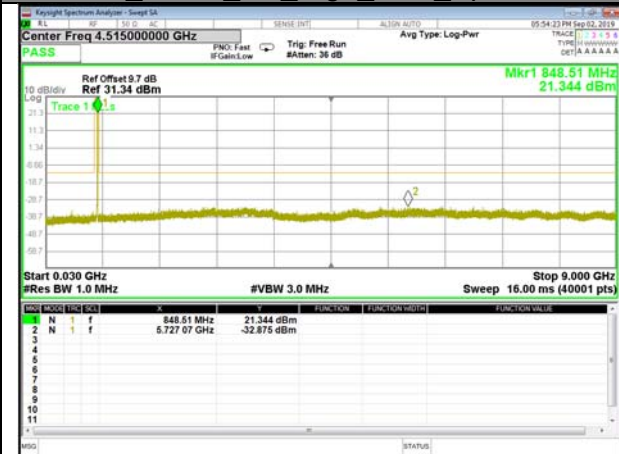
B26_QPSK_5M_High_CDT_Spurious
