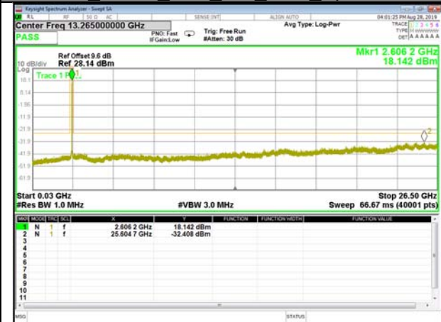
B41_QPSK_10M_High_CDT_Spurious
