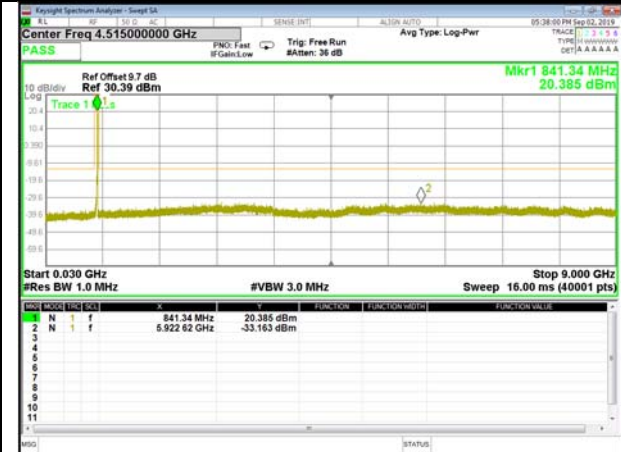
B26_QPSK_10M_High_CDT_Spurious
