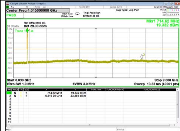
B17_Q16_10M_High_CDT_Spurious
