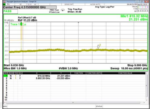
B26_Q16_3M_Low_CDT_Spurious
