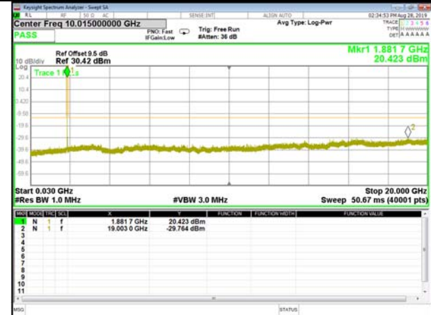
B25_QPSK_3M_High_CDT_Spurious
