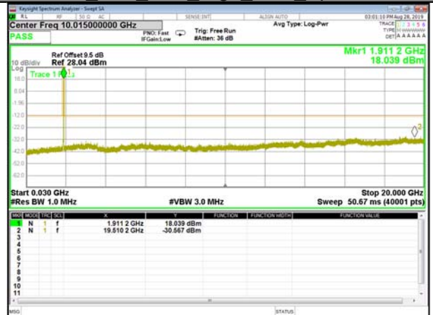
B25_Q16_10M_High_CDT_Spurious
