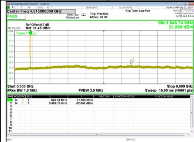
B26_QPSK_1.4M_High_CDT_Spurious
