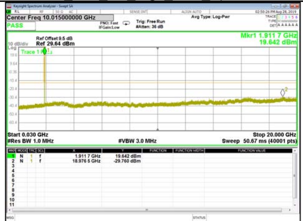
B25_Q16_5M_High_CDT_Spurious
