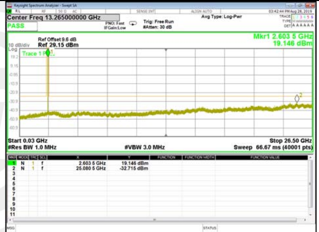
B41_Q16_5M_High_CDT_Spurious
