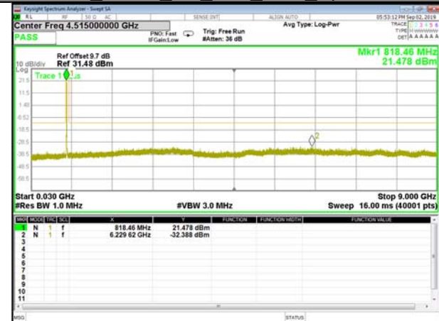
B26_QPSK_5M_Low_CDT_Spurious
