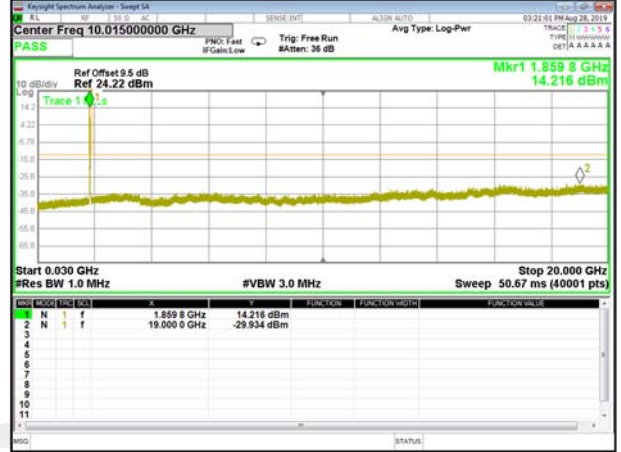
B25_Q16_20M_Mid_CDT_Spurious
