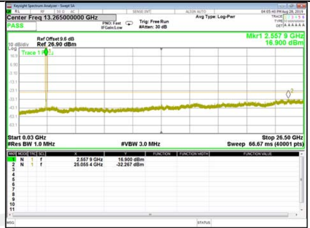
B41_Q16_10M_Mid_CDT_Spurious
