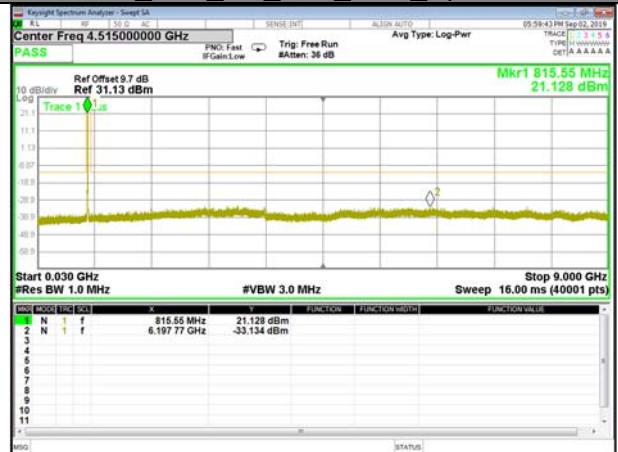
B26_Q16_5M_Low_CDT_Spurious
