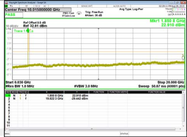
B25_Q16_1.4M_Mid_CDT_Spurious
