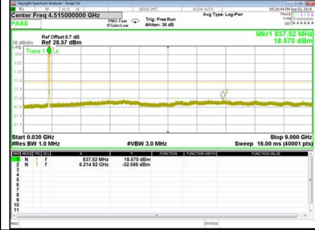
B26_QPSK_15M_High_CDT_Spurious
