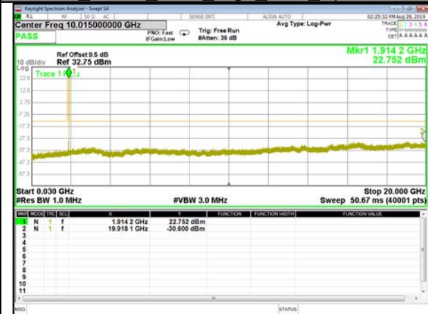
B25_QPSK_1.4M_High_CDT_Spurious
