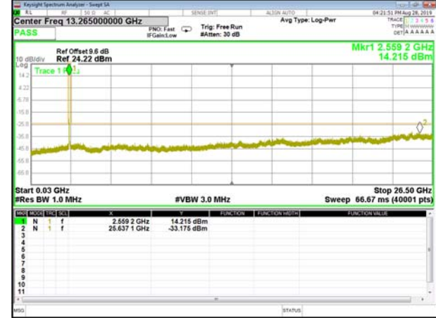
B41_QPSK_20M_Mid_CDT_Spurious
