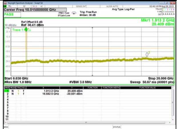
B25_Q16_3M_High_CDT_Spurious
