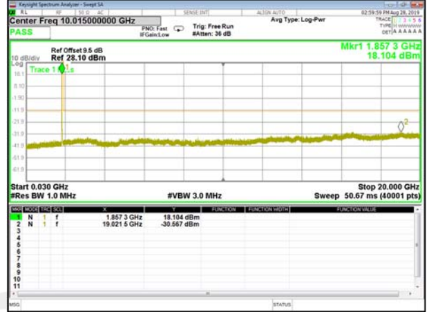
B25_Q16_10M_Mid_CDT_Spurious
