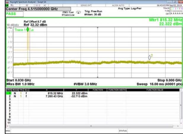
B26_QPSK_3M_Low_CDT_Spurious
