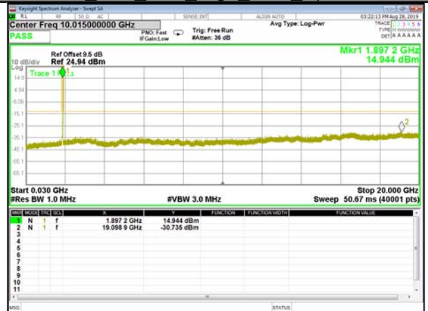
B25_Q16_20M_High_CDT_Spurious
