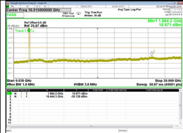
B25_QPSK_20M_High_CDT_Spurious
