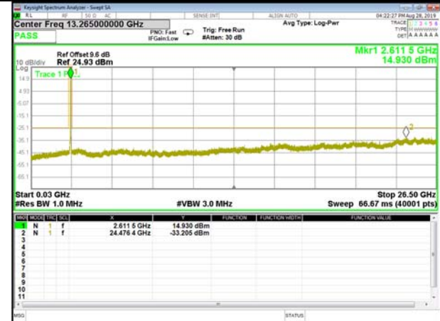
B41_QPSK_20M_High_CDT_Spurious
