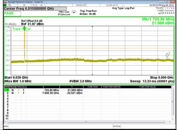
B17_Q16_5M_Mid_CDT_Spurious
