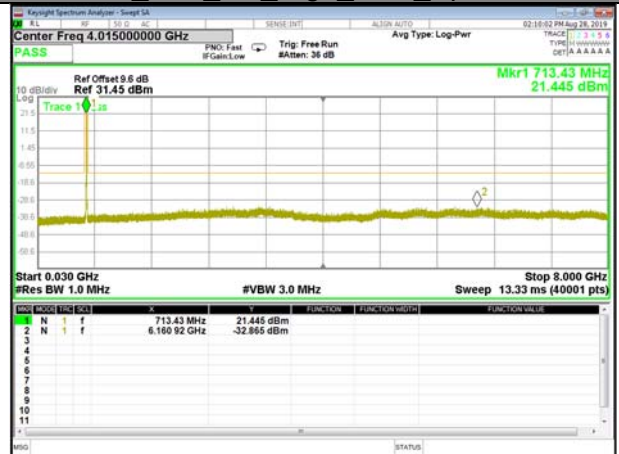
B17_Q16_5M_High_CDT_Spurious
