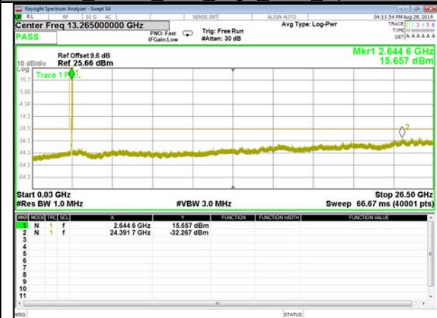
B41_QPSK_15M_High_CDT_Spurious
