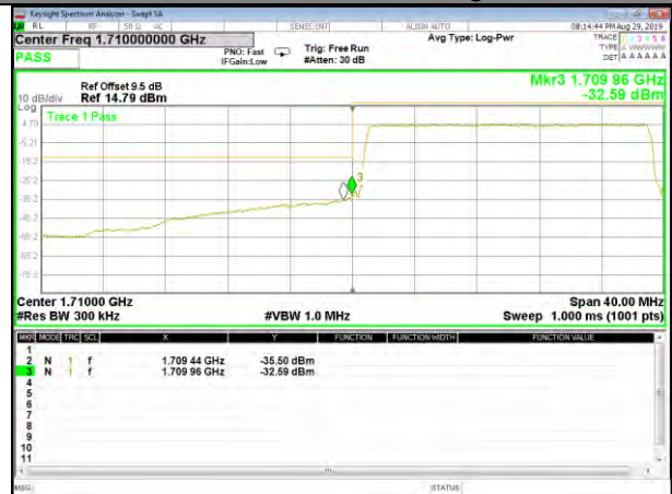
QPSK_20M_Lower_Band edge_Full-RB
