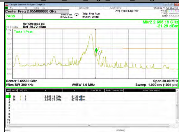
B41_Q16_15M_High_1-RB_Bedge
