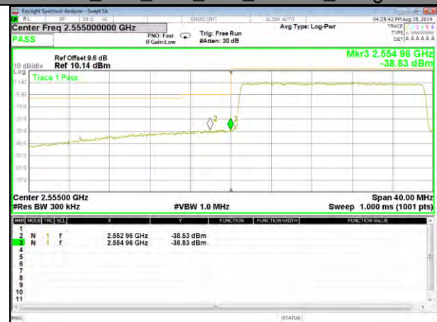
B41_Q16_20M_Low_Full-RB_Bedge
