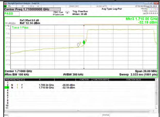
16QAM_10M_Lower_Band edge_Full-RB
