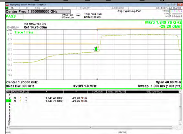
B25_QPSK_20M_Low_Full-RB_Bedge
