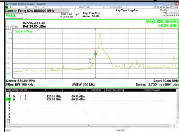
B26_QPSK_15M_High_1-RB_Bedge
