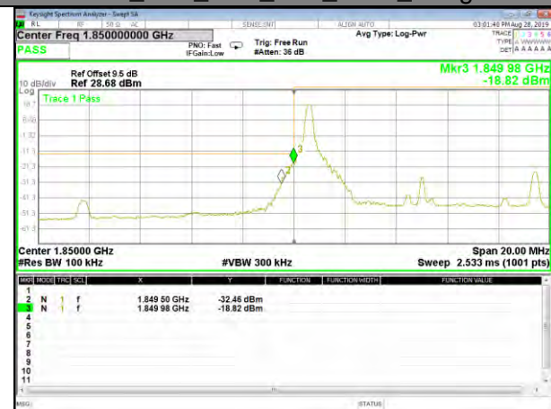
B25_Q16_10M_Low_1-RB_Bedge
