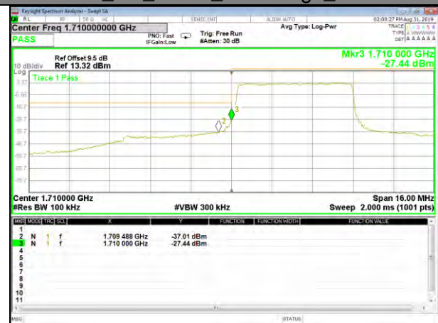
QPSK_5M_Lower_Band edge_Full-RB
