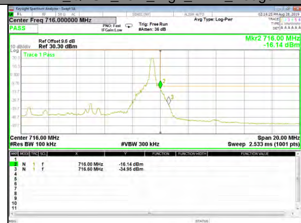
B17_QPSK_10M_High_1-RB_Bedge
