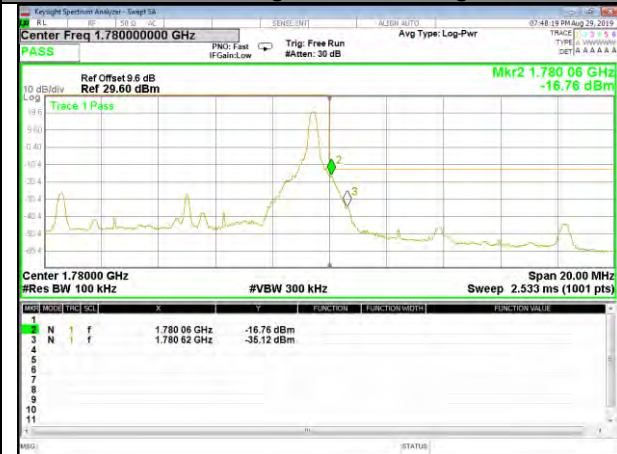
16QAM_10M_Lower_Band edge_1-RB
