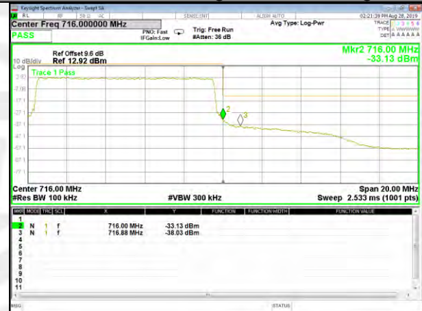
B17_Q16_10M_High_Full-RB_Bedge
