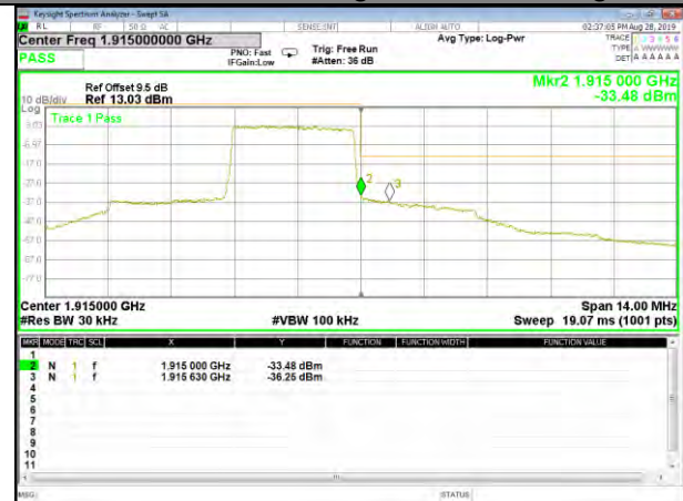
B25_QPSK_3M_High_Full-RB_Bedge
