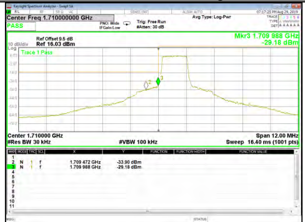
16QAM_1.4M_Lower_Band edge_Full-RB
