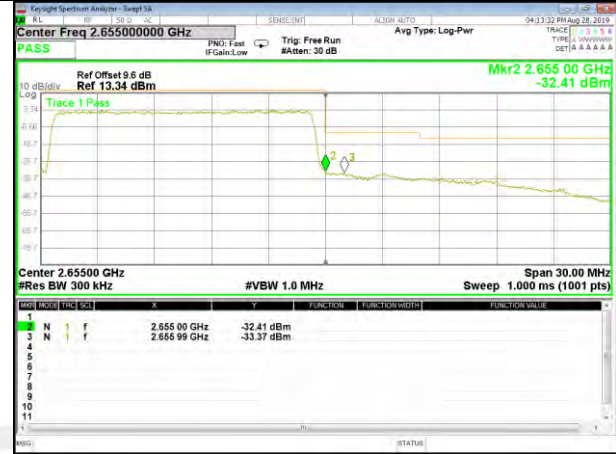
B41_Q16_15M_Low_Full-RB_Bedge
