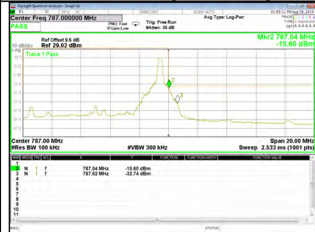
B13_Q16_10M_High_1-RB_Bedge
