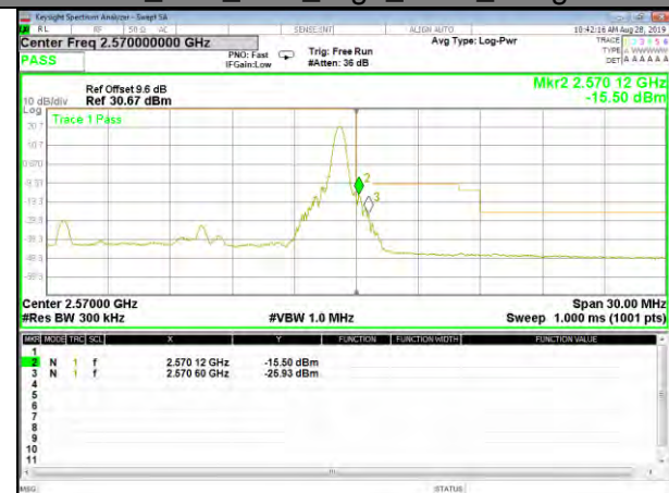
B7_Q16_15M_High_1-RB_Bedge
