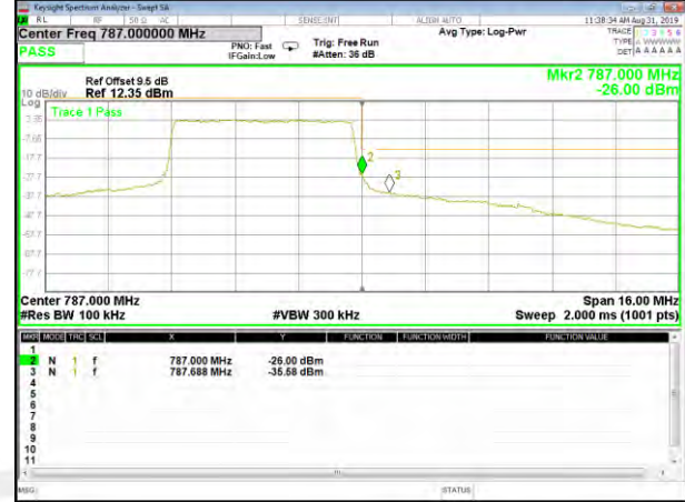
B13_QPSK_10M_Low_Full-RB_Bedge
