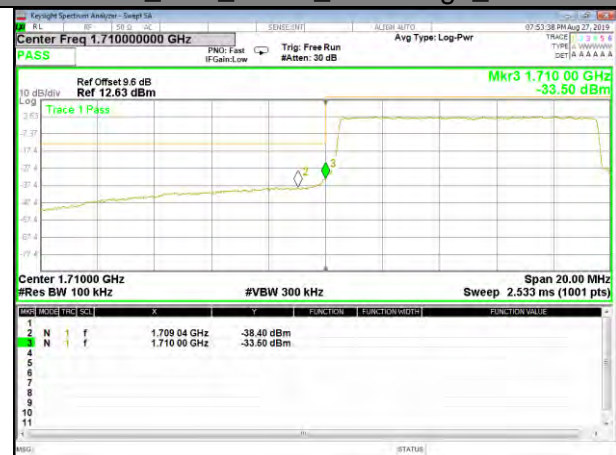
16QAM_10M_Lower_Band edge_Full-RB
