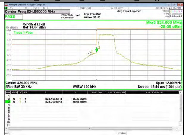
B5_Q16_1.4M_Low_Full-RB_Bedge
