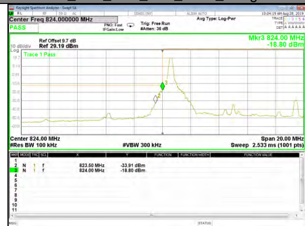
B5_Q16_10M_Low_1-RB_Bedge
