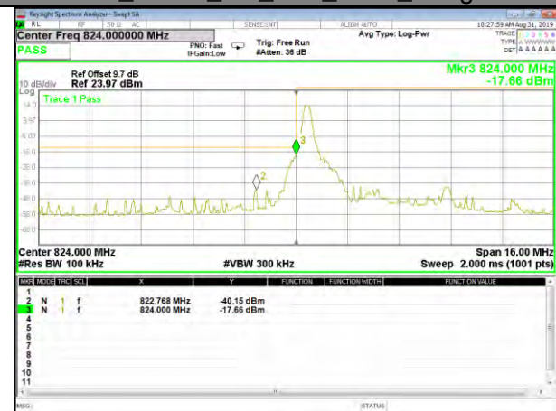
B5_QPSK_5M_Low_1-RB_Bedge
