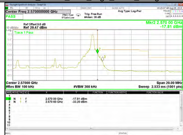
B7_QPSK_10M_High_1-RB_Bedge
