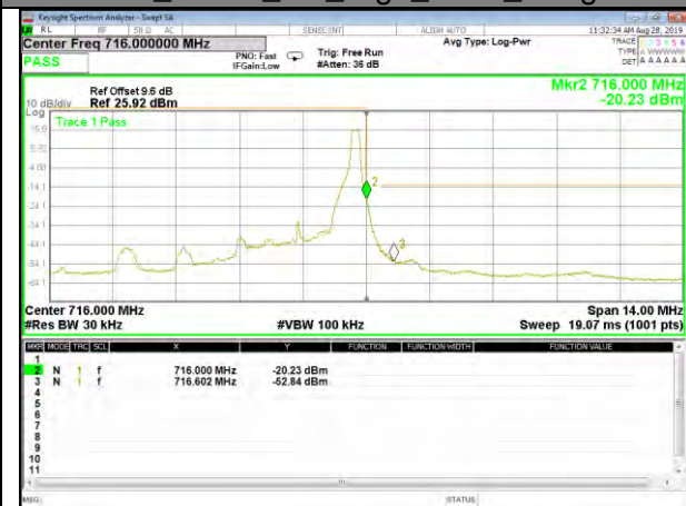
B12_QPSK_3M_High_1-RB_Bedge
