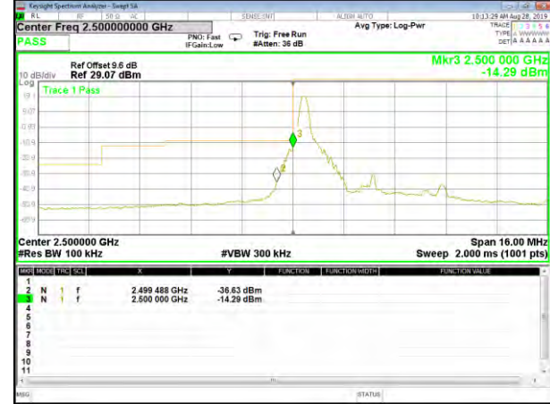
B7_QPSK_5M_High_1-RB_Bedge
