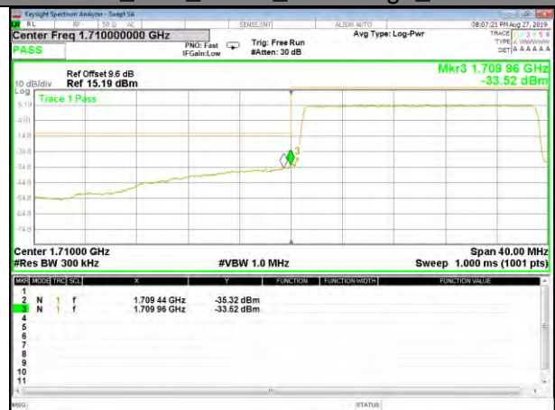
QPSK_20M_Lower_Band edge_Full-RB
