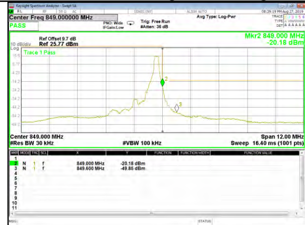
B5_Q16_1.4M_Low_1-RB_Bedge
