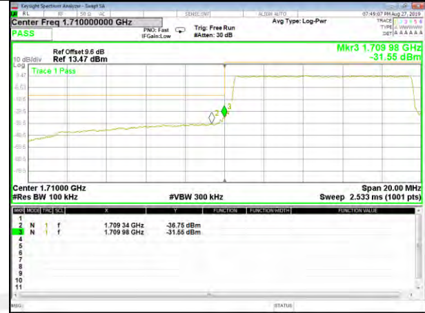
QPSK_10M_Higher_Band edge_Full-RB
