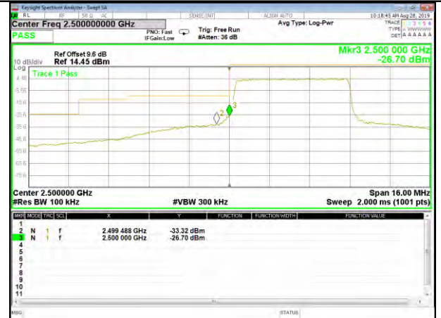
B7_Q16_5M_Low_Full-RB_Bedge
