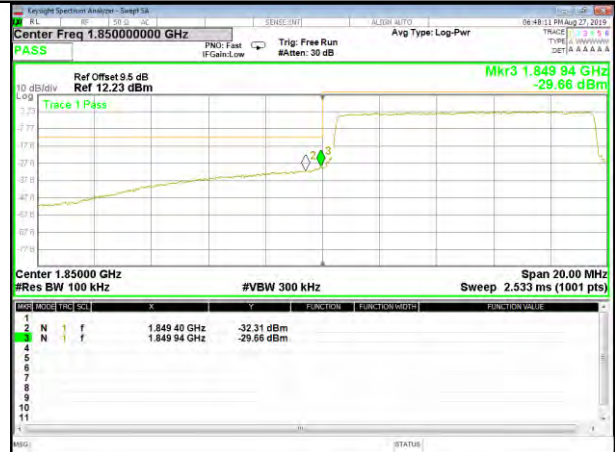
16QAM_10M_Lower_Band edge_Full-RB
