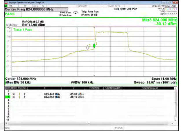
B5_Q16_3M_High_Full-RB_Bedge
