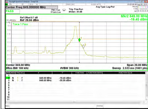
B5_Q16_10M_High_1-RB_Bedge
