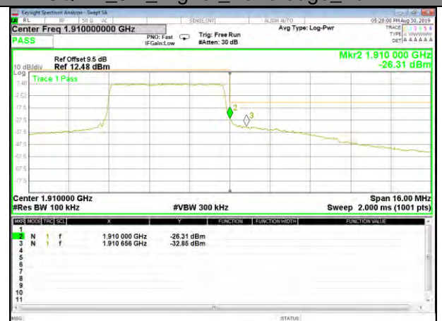
16QAM_5M_Higher_Band edge_Full-RB
