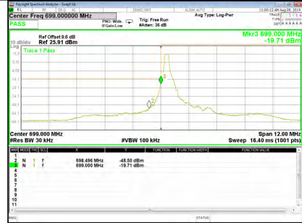
B12_QPSK_1.4M_High_1-RB_Bedge
