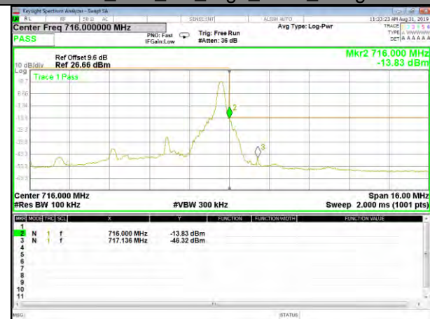
B12_Q16_5M_High_1-RB_Bedge
