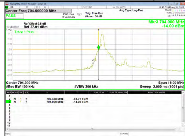
B17_Q16_5M_Low_1-RB_Bedge
