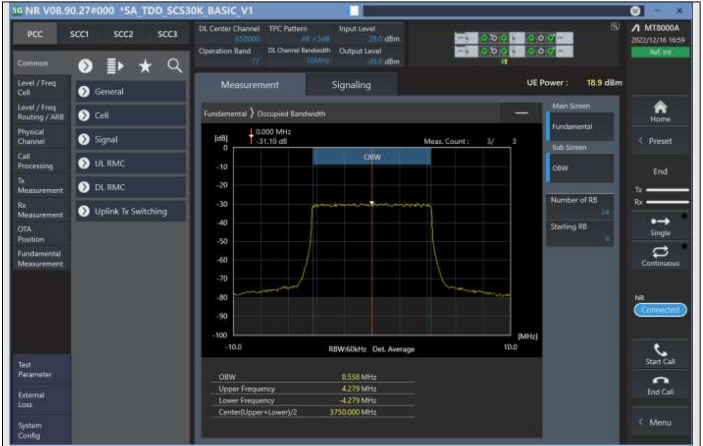
n77_10MHz_30kHz_650000_DFT-s-OFDM 256QAM_Outer_Full
