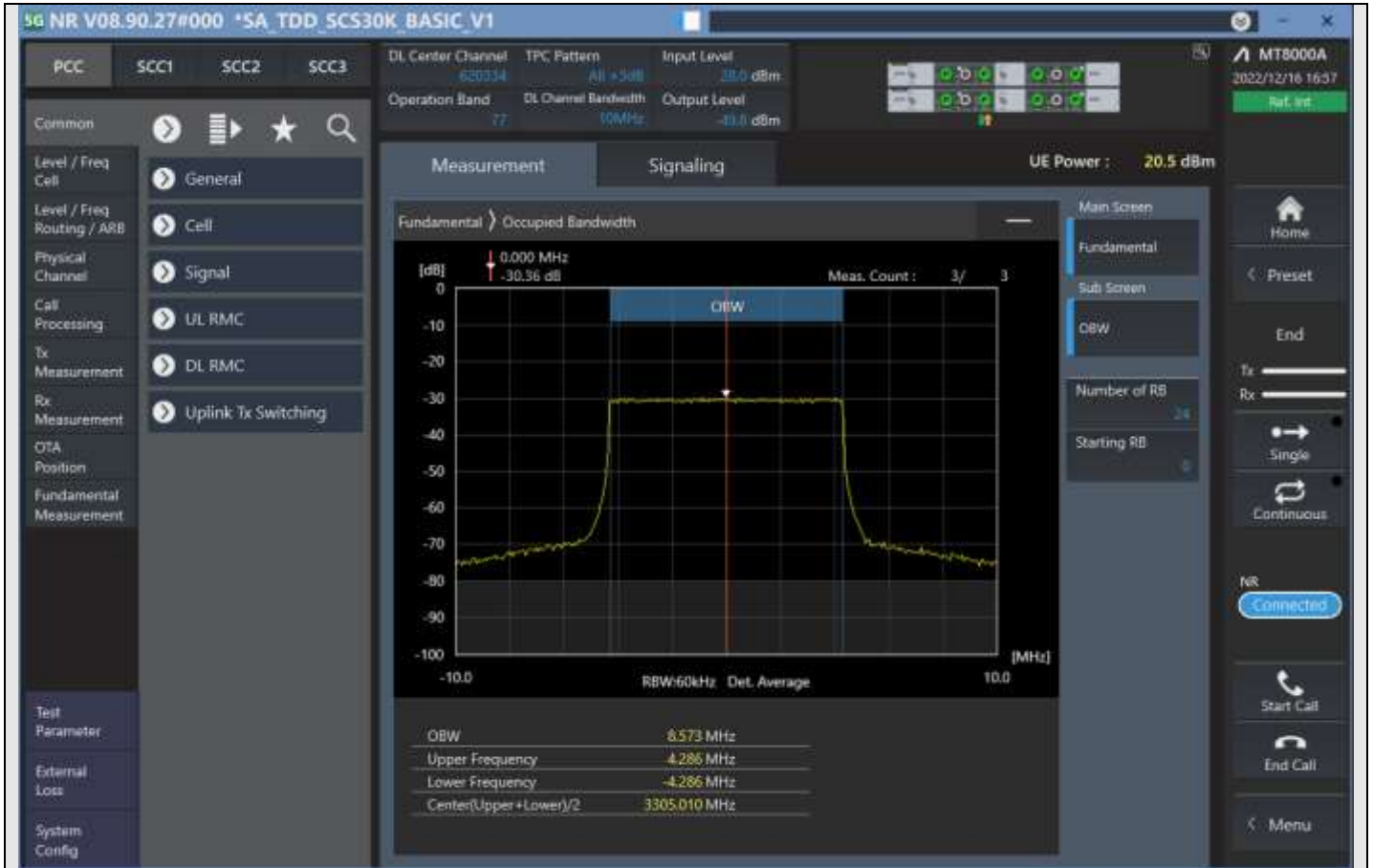
n77_10MHz_30kHz_620334_CP-OFDM 16QAM_Outer_Full
