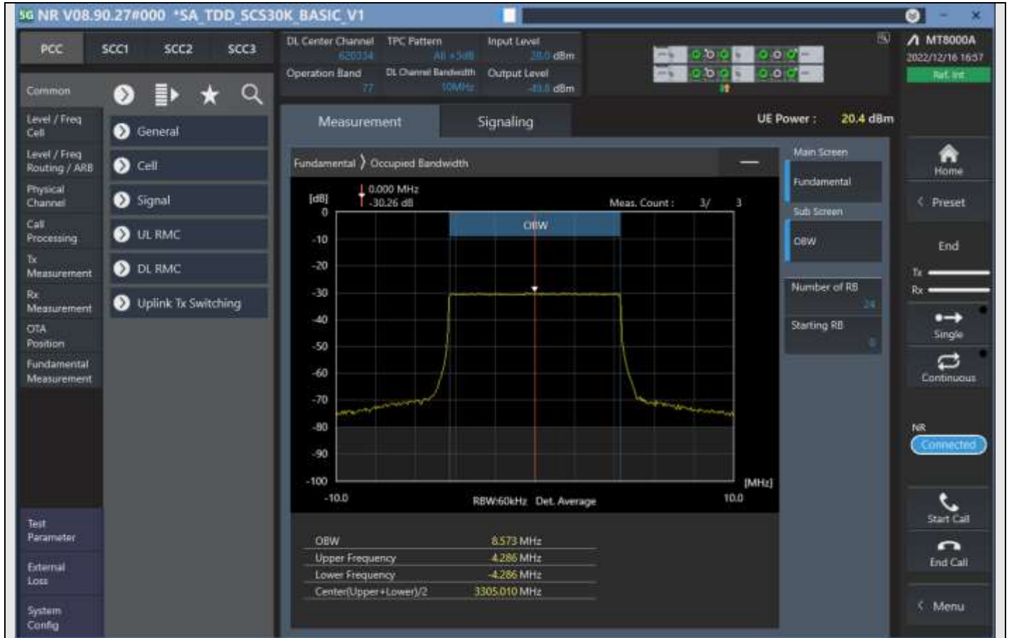
n77_10MHz_30kHz_620334_CP-OFDM QPSK_Outer_Full
