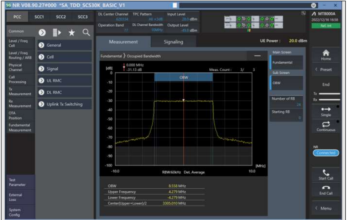
n77_10MHz_30kHz_620334_CP-OFDM 64QAM_Outer_Full
