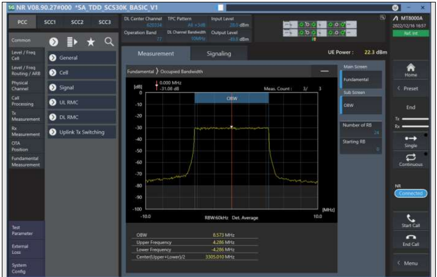
n77_10MHz_30kHz_620334_DFT-s-OFDM QPSK_Outer_Full
